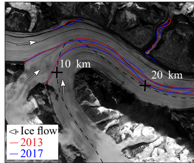
(b) Moraine positions
