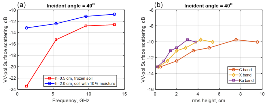
Figure 5. (a) Backscattering at VV polarization as a function of frequency: red curve is results with frozen soil (permittivity 4 + 1i ) and rms height of 0.5 cm, and blue curve is results with soil of 10 % moisture and rms height of 2 cm. (b) Backscattering at VV polarization as a function of rms height with soil of 10 % moisture at C-, X-, and Ku-band.
