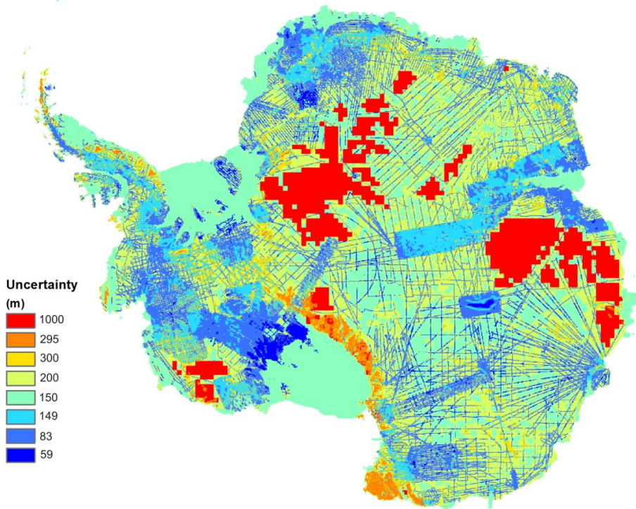
Fig. 11. Estimated uncertainty in ice thickness grid.
