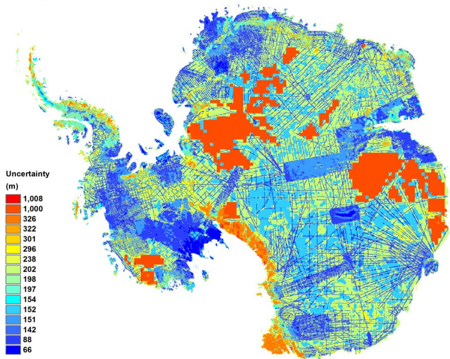
Fig. 12. Estimated uncertainty in bed elevation grid.
