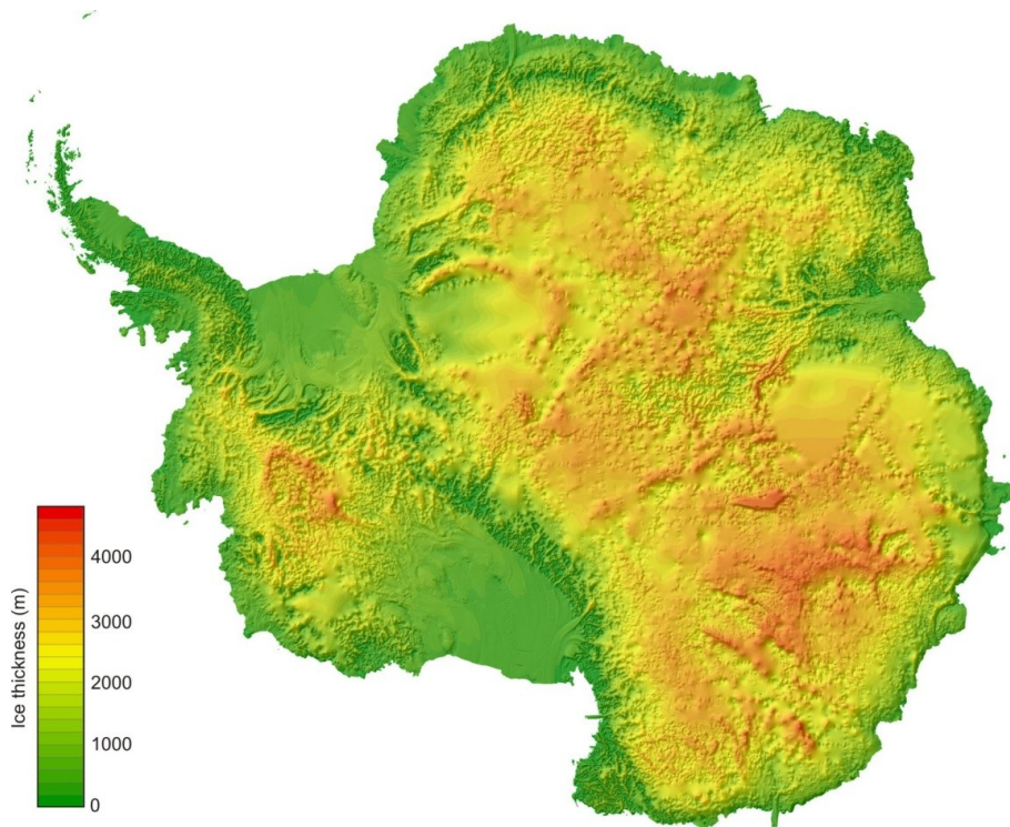
Fig. 8. Bedmap2 ice thickness grid.
