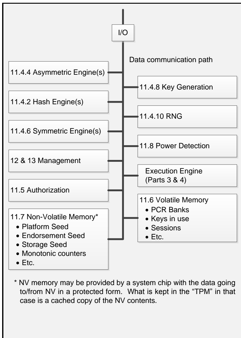
Figure 2 — Architectural Overview
