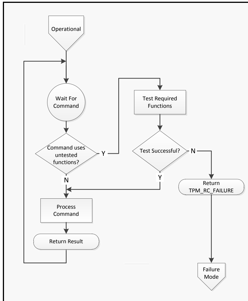
Figure 6 — On-Demand Self-Test
