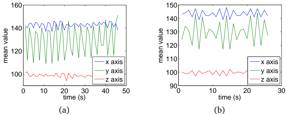
Figure 5.5: The 1Hz mean acceleration values from 15 barbell curls in (a) normal workout speed and (b) very fast workout speed.
