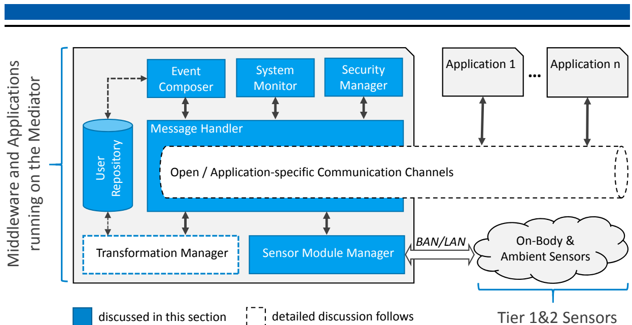
Figure 3.1: Event-driven middleware architecture consisting of an Event Composer for reasoning such as deriving sensor fidelity information, a System Monitor for keeping track of the overall system status, a Security Manager for encryption, verification, and managing permissions, a User Repository storing user specific data, a Message Handler for message passing, a Transformation Manager for converting sensor data to the desired representation, and a Sensor Module Manager that administers sensor connections.
