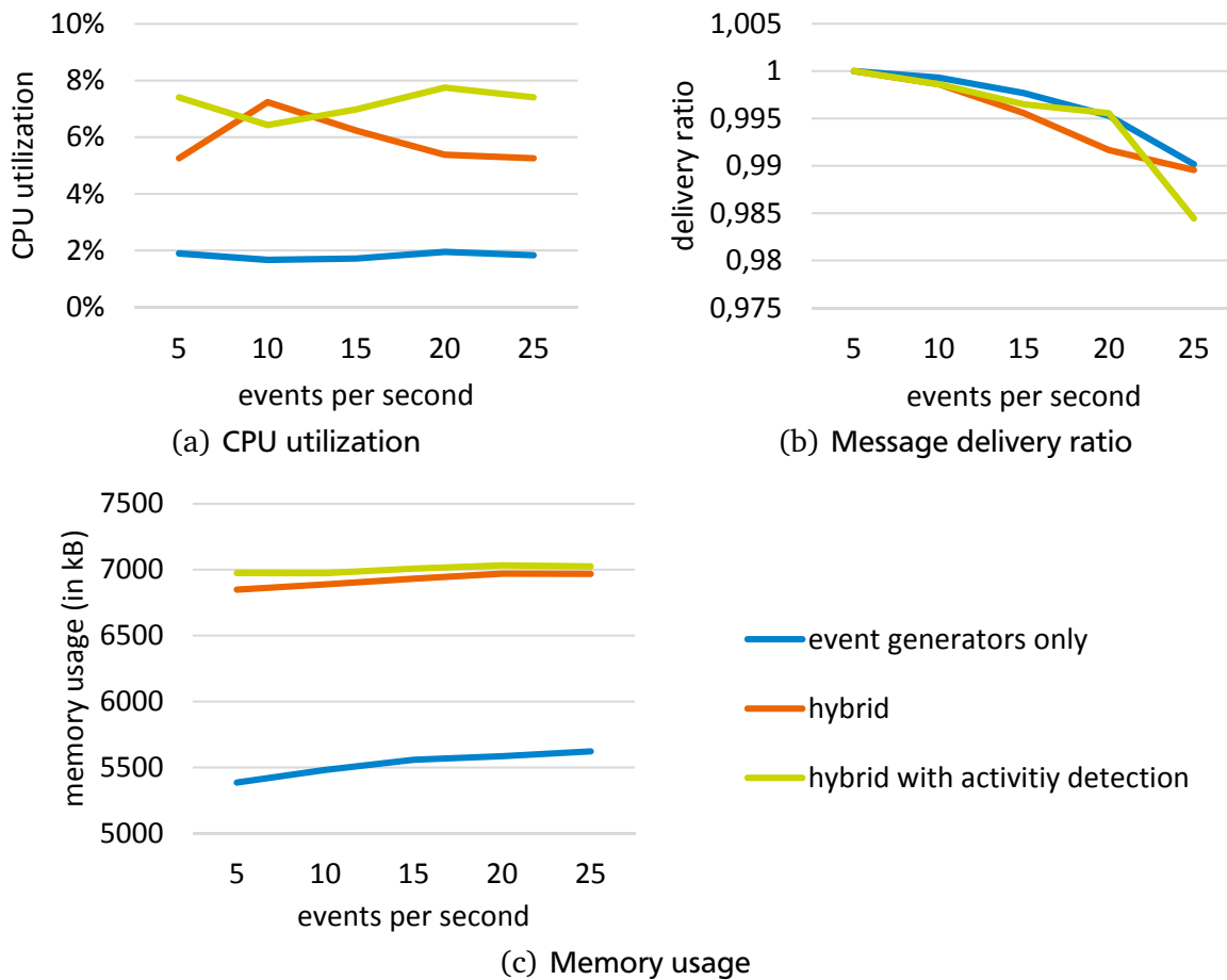
Figure 6.3: Comparison of the system's performance for: I) event generators only, II) a hybrid setup, consisting of an increasing amount of event generators as well as a Bluetooth heart rate sensor and a Bluetooth accelerometer, and III) the hybrid setup plus activity recognition as described in Section 5.1.2.
