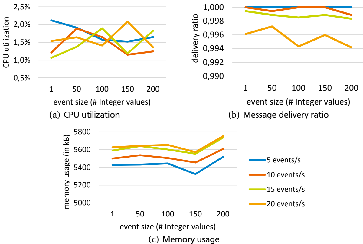
Figure 6.4: Increasing payload size from 1 to 200 Integer values per event and different workload configurations. In addition to the payload, each event consists of an ID, type, timestamp, producer ID, sensor type, and time of measurement.
