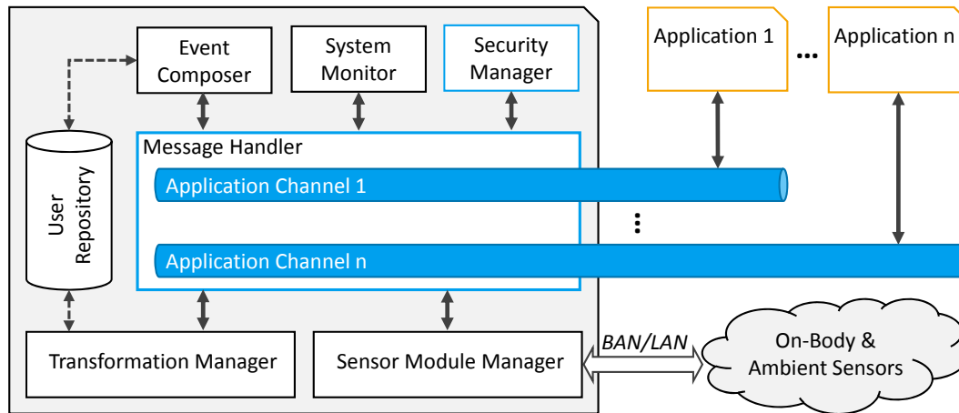
Figure 3.4: Middleware architecture with application-specific communication channels that allow secure communication and a tailor-made event delivery. Each application sends subscription and advertise messages to the Message Handler which, in turn, establishes the tailored communication channels.
