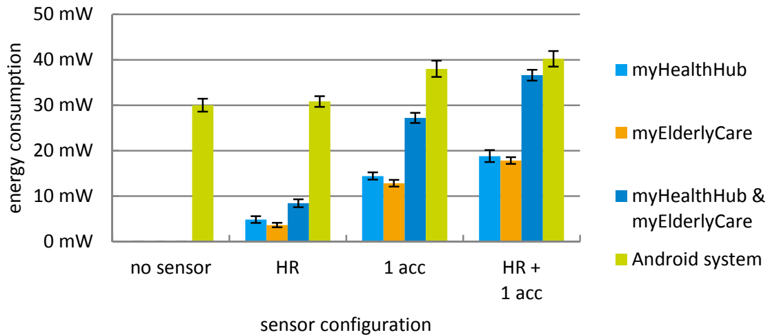
Figure 6.1: Energy consumption of the myElderlyCare application for different sensor configurations. By connecting a heart rate (HR) sensor, the application monitors the wearer’s heart rate. Connecting an accelerometer (acc) enables the recognition of daily activities (cp. Section 5.1.2).
