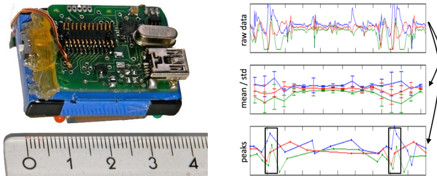
Figure 5.3: The Porcupine inertial units were designed to operate as long as possible on a light-weight battery. A dedicated microcontroller calculates basic statistics and the peak features on-board before transmitting them wirelessly to the smartphone.
