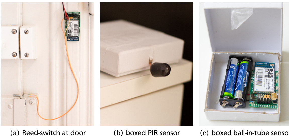
Figure 5.17: Wi-Fi modules with sensors attached. The first picture shows a Reed-switch attached to a door. The second picture shows a cased modules with a PIR sensor attached (black device). Figure 5.17(c) depicts how a Wi-Fi module with two AAA batteries and a ball-in-tube sensor are placed in their casing.
