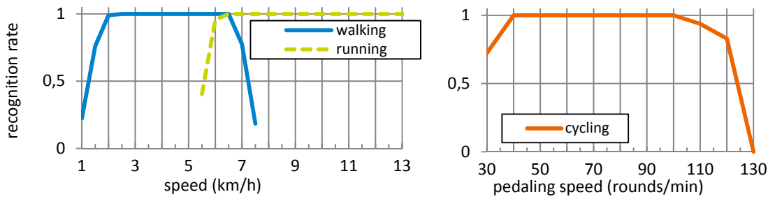
Figure 5.4: Stress-testing the daily activity recognition: Accuracy for different speeds, showing the regions where the activities are reliably detected.
