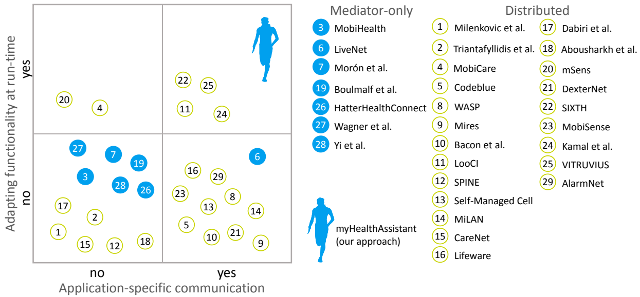
Figure 2.2: Comparison of our work (myHealthAssistant) with related work by focusing on two contributions of our work: application-specific communication and adapting functionality at run-time . A distinction is made between distributed approaches that run on multiple sensor nodes (green circles) and mediator-only approaches running on a single device (blue points). Our approach is the only mediator-only system operating on off-the-shelf sensors that provides both features.
