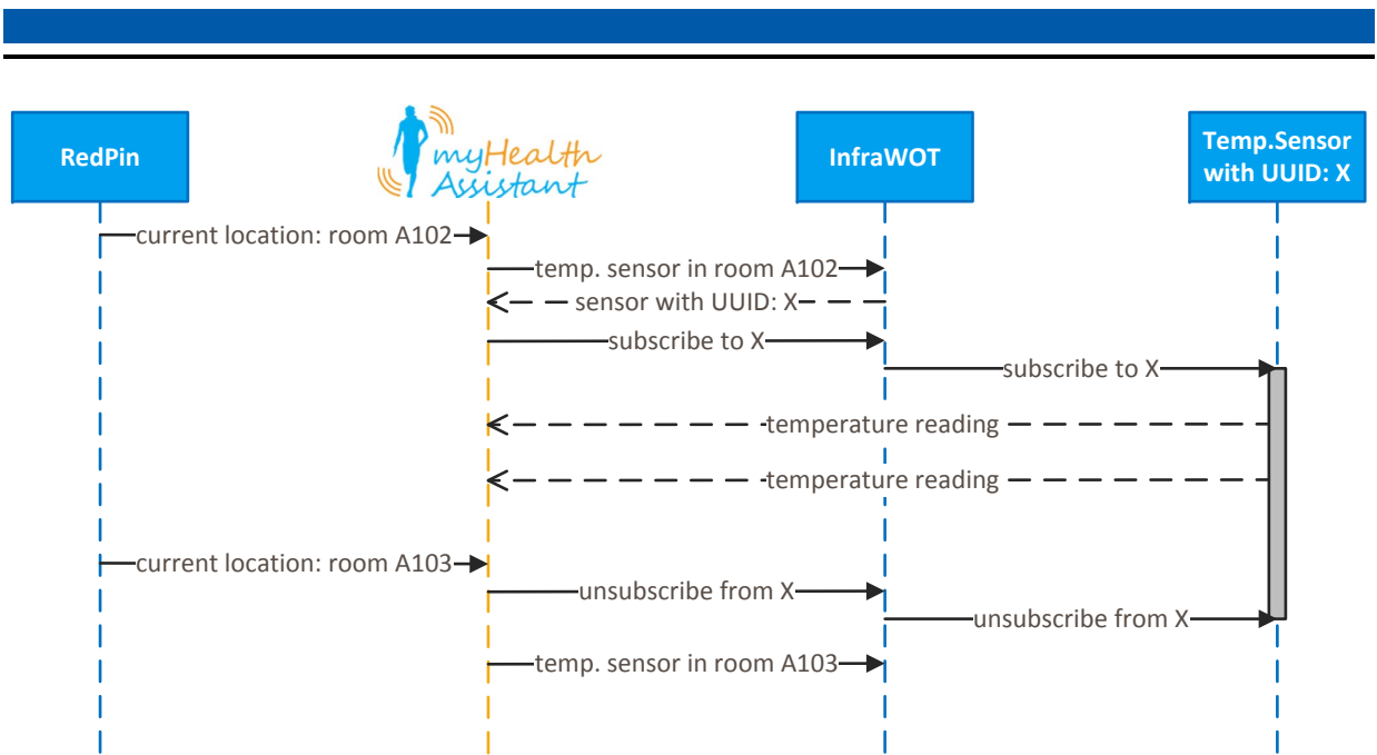
Figure 4.7: Sequence diagram showing the interaction among RedPin, myHealthHub (myHealthAssistant), InfraWOT, and ambient sensors.
