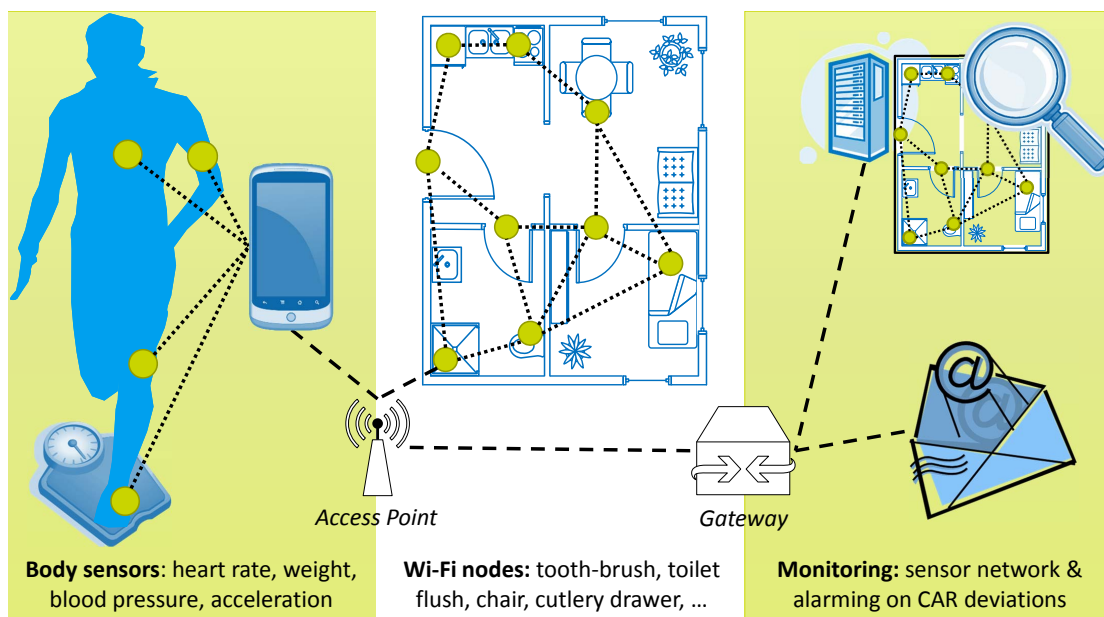
Figure 5.16: System setup of the myElderlyCare application consisting of Bluetooth on-body sensors and Wi-Fi environmental sensors. The environmental sensors are used for detecting deviations in the circadian activity rhythm (CAR) and alarming via e-mail. Heartbeat messages sent from the BASN allows monitoring the system's liveliness.
