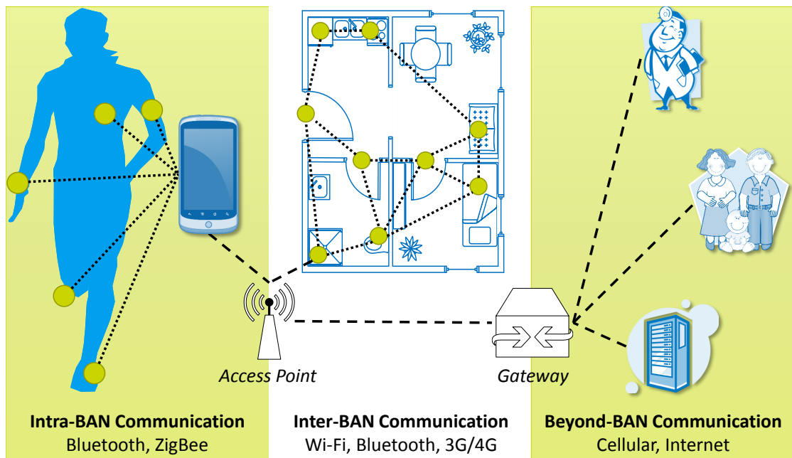
Figure 2.1: Communication in a 3-tier Body Area Network (BAN): body sensors communicate via intra-BAN communication among each other and with a mediator device, inter-BAN communication among BSNs and the environment including ambient sensors, beyond-BAN communication with care-givers and remote repositories.
