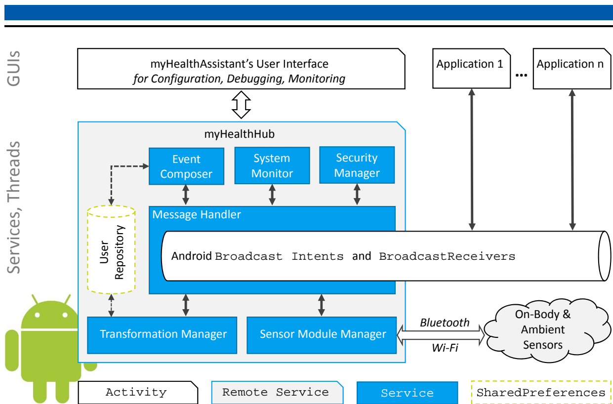
Figure 4.2: Implementation of the event-driven middleware for body and ambient sensor networks as Android Services. The implemented modules correspond to the modules presented in Chapter 3. Bluetooth and Wi-Fi is used for communicating with on-body and ambient sensors and Android Activities provide a user interface for configuring the middleware. Android Broadcast Intents and Broadcast Receivers are used for inter-application communication.
