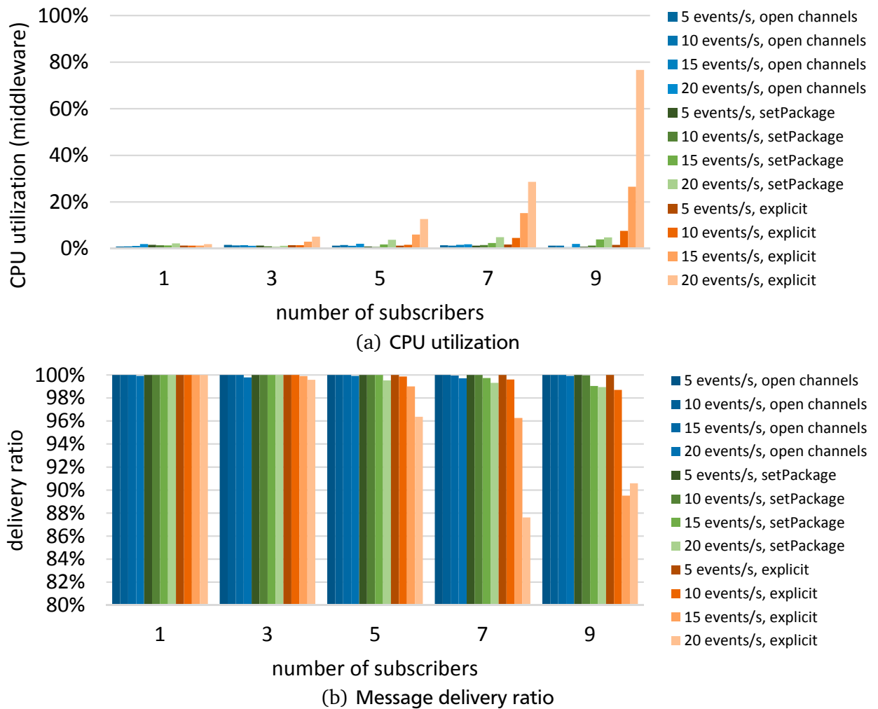
Figure 6.5: Performance evaluation of three Message Handler implementations: I) open communication channels, II) implicit broadcasts Intents using the setPackage option, and III) explicit broadcast Intents. For all implementations up to 9 subscribers and a workload of 5, 10, 15, and 20 events per second are tested. The explicit addressing performs the worst.
