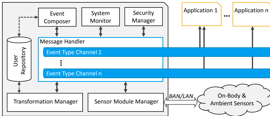
Figure 3.2: Middleware architecture with open event channels (highlighted in blue) implemented in the Message Handler. Events are distributed in multiple channels with respect to their event type. By subscribing to one or more open event channels, applications receive event notifications as shown by the arrows from the event channels to the individual applications.
