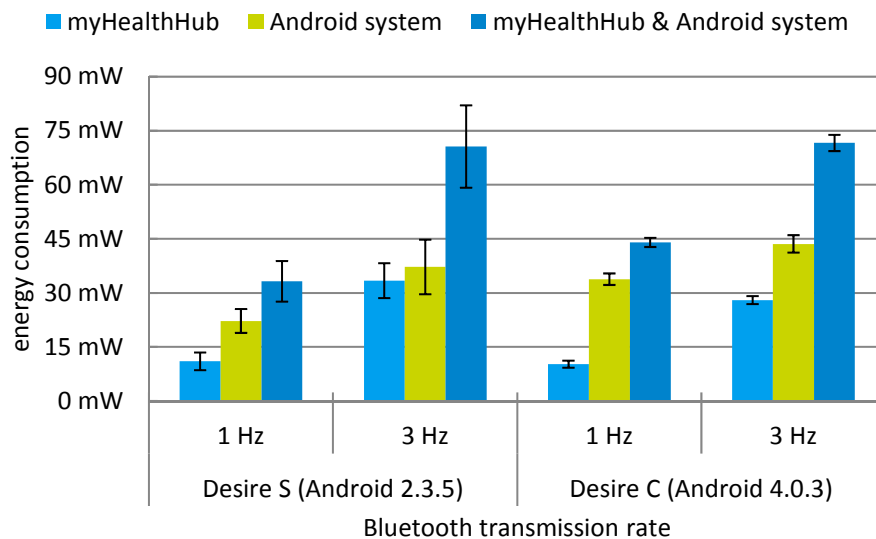
Figure 6.2: Energy consumption for two different Bluetooth transmission rates (1 Hz versus 3 Hz). Increasing the transmission rate drastically increases the overall energy consumption.
