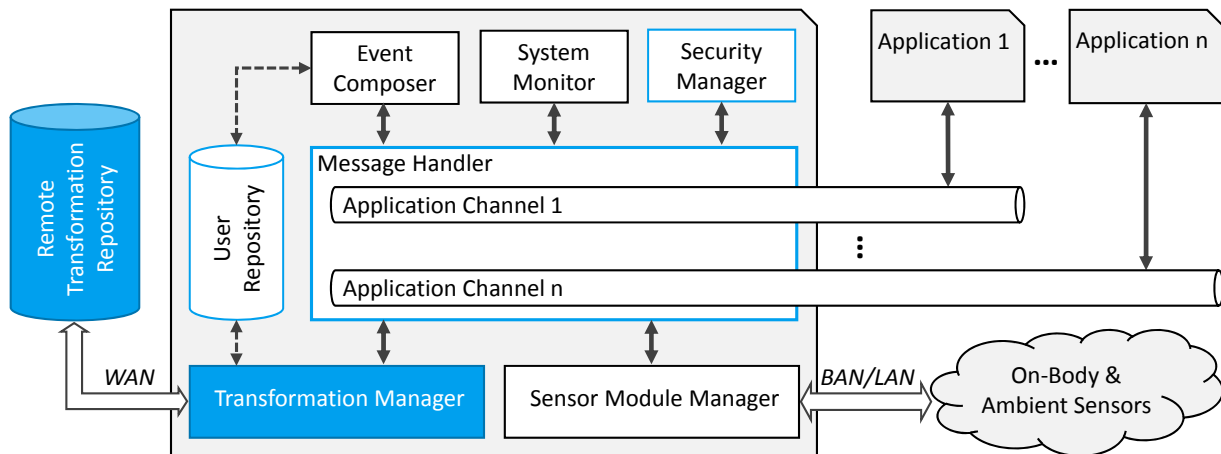
Figure 3.5: The middleware’s Transformation Manager (blue) receives transformation requests from the Message Handler. Upon an incoming request, it checks whether it has a matching transformation locally installed. If this is not the case, the request is forwarded to the Remote Transformation Repository (blue) and a matching transformation downloaded at run-time.
