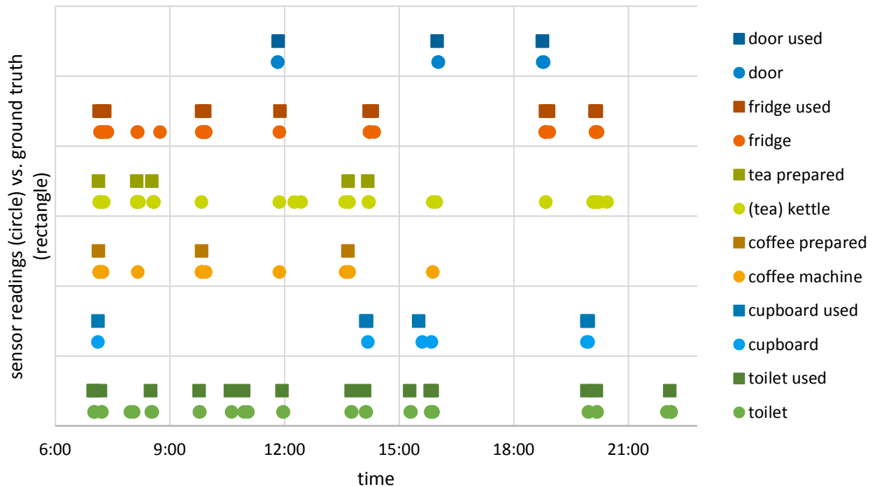
Figure 5.20: Classification of events based on simple rules that map the interaction with an object to an activity. The rectangles are the ground truth data given by the participants and circles are sensor readings. The overall precision is 68.6% and the overall recall 100% for a 10 minutes suppression of re-occurring events.
