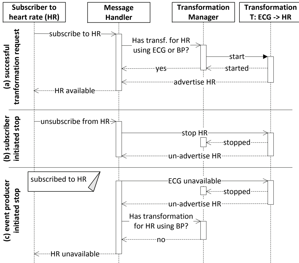
Figure 3.7: Sequence diagram illustrating the communication among software components for starting and stopping an event transformation: (a) installing an event transformation for transforming events of type ECG to type HR, (b) the event transformation is stopped because the last subscriber to HR unsubscribed, (c) the event transformation is stopped because the event producer for events of type ECG is no longer available.
