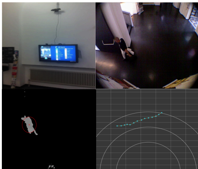
Figure 1 – Audience Monitoring Tool for Public Displays. Top left: Kinect sensor mounted on the wall above the existing public display. Top right: View of the scene from the sensor (video was recorded only during the evaluation). Bottom left: Depth view of the scene and detection of passer's-by presence. Bottom right: Visualization of the passer's-by path.
