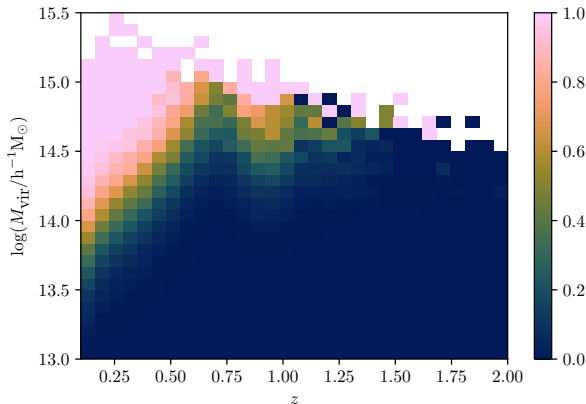
Figure 1: Distribution of the clusters selected in the Flagship dark matter halo catalog. We set the S/N ( q_{\text{obs}} = 6 , from equation 9), so that we remove most of the low mass systems for which the uncertainties are high, especially regarding the selection function. The color scale represents the fraction of detected clusters.
