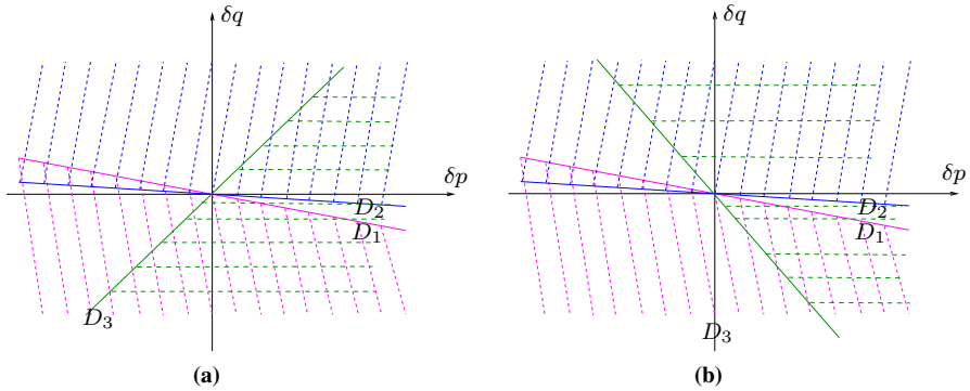
Fig. 6 Description of the analysis for \omega_M \preceq k_M
