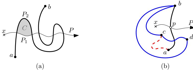
Figure 5: (a) and (b) give an illustration of the proof of Theorem 2.
