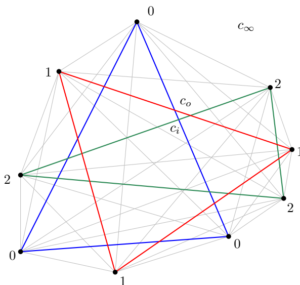
Figure 6: A cell-convex drawings of K_9 . If the cell c_o is chosen as the outer cell, then Colorful Carathéodory theorem does not hold for the colored triangles and every point x from the cell c_i . The special cell of the pseudolinear drawing is marked c_\infty .
