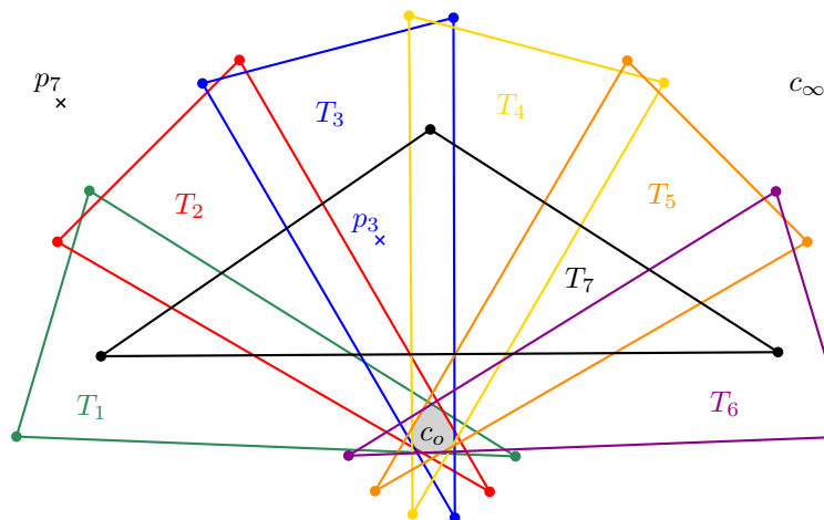
Figure 7: A drawing D of K_{21} is obtained by adding the remaining edges as straight-line segments. Making the gray cell c_o the outer cell, we obtain a cell-convex drawing with Helly number 7.
