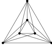
Figure 9: The unique topological drawing of K_6 which has the minimum of 3 crossings.
