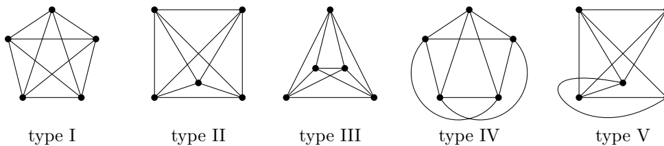
Figure 8: The five types of topological drawings of K_5 .
