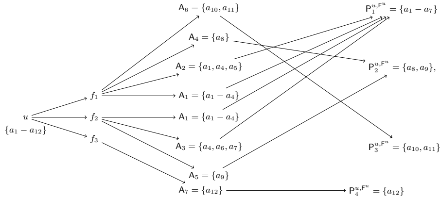
Fig. 15: Example for collateral information collection while enabling profiling to P_j
