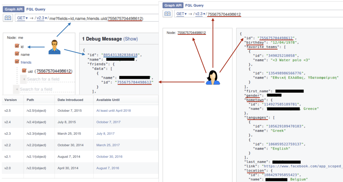
Fig. 2: Collateral information collection example of v2.0 – v2.3 of the API (upper left and right) and the Facebook Graph API versioning history (bottom left).
