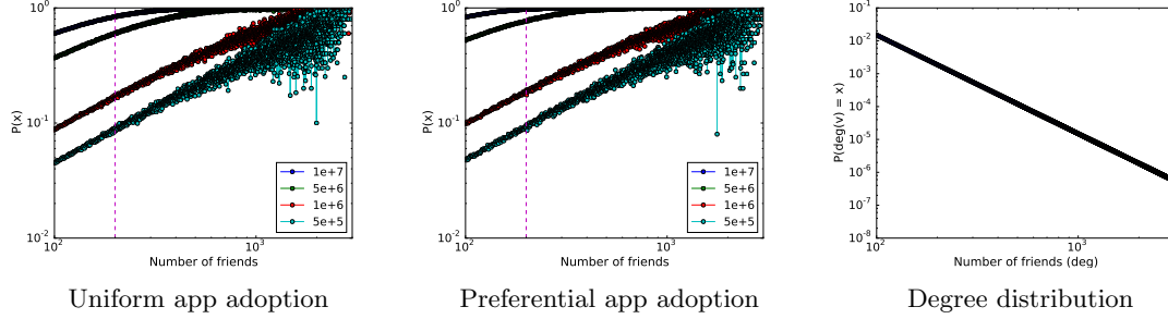
Fig. 12: Simulation results on a BA graph with k = 1,000,000 and d = 200
