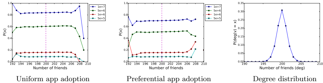
Fig. 14: Simulation results on a WS graph with k = 1,000,000 and d = 200
