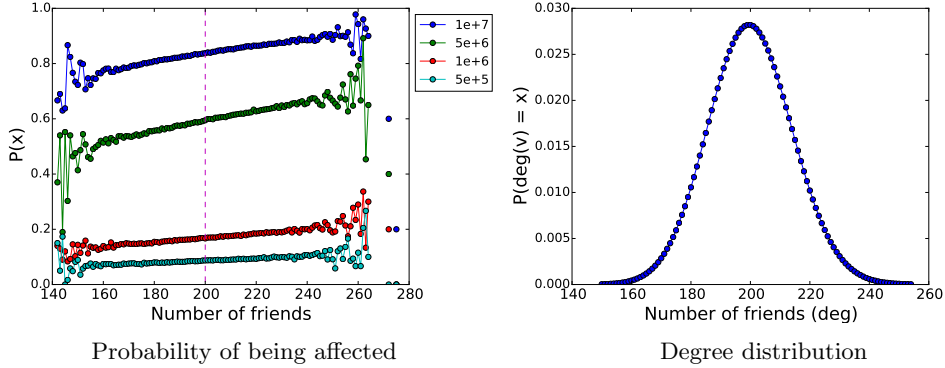
Fig. 10: Simulation results on an ER graph with k = 1,000,000 and d = 200
