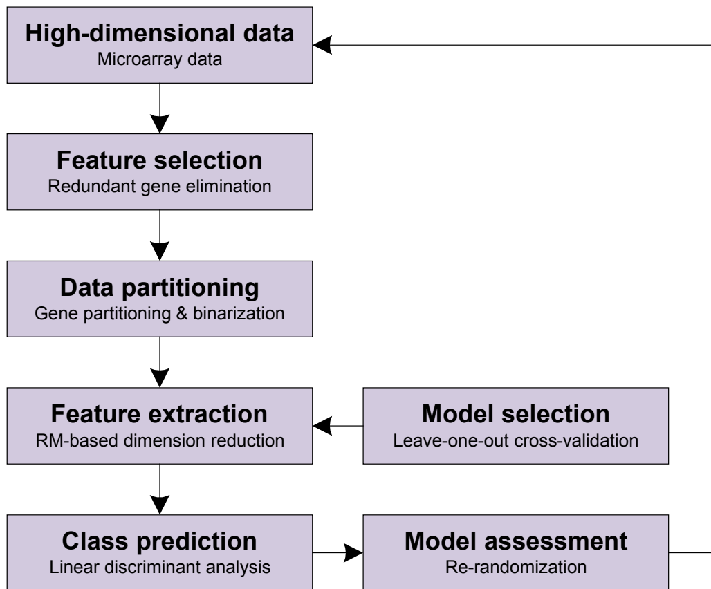
Figure 1: The framework of dimension reduction.
