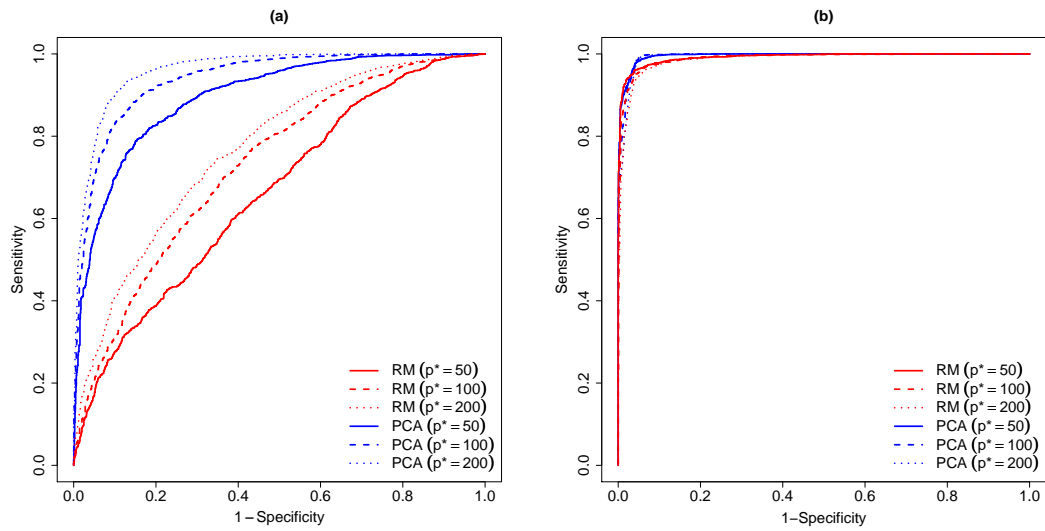
Figure 3: Receiver operating characteristic curves (ROC) for RM- and PCA-based prediction models using random (a) and supervised (b) gene selection on the Leukemia data set with 36/36 split of samples over 100 randomization trials.
