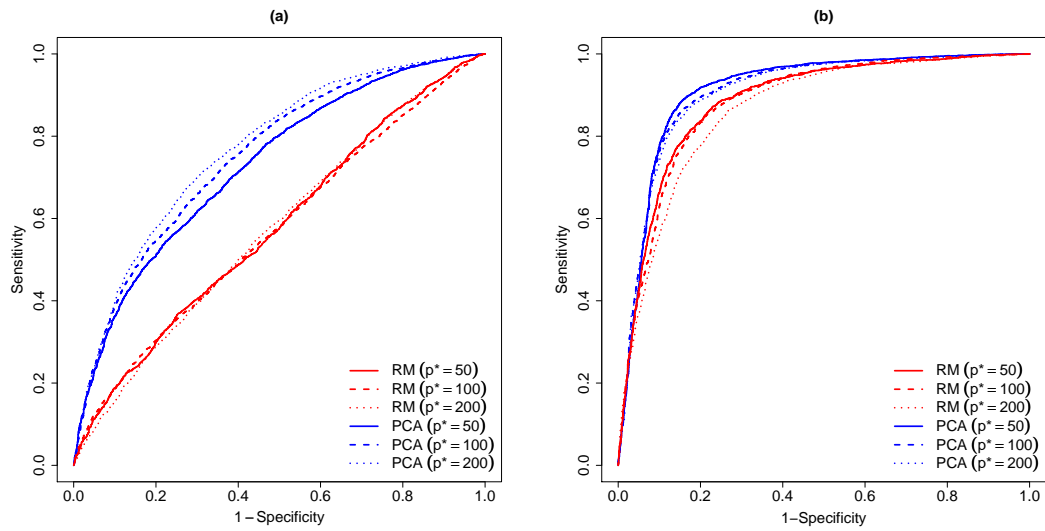
Figure 4: Receiver operating characteristic curves (ROC) for RM- and PCA-based prediction models using random (a) and supervised (b) gene selection on the Prostate data set with 36/66 split of samples over 100 randomization trials.
