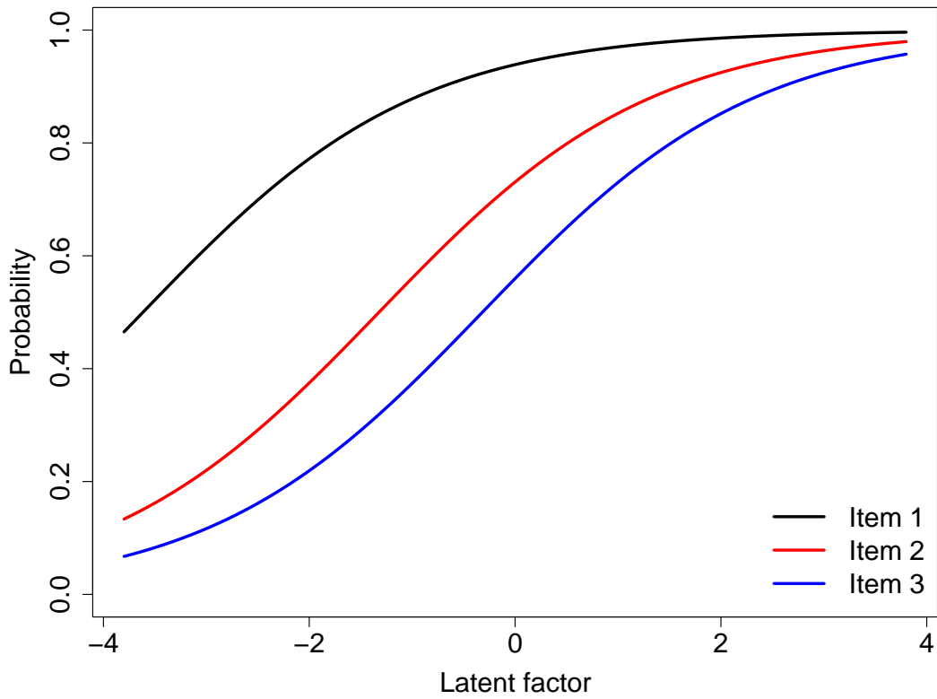
Figure 2: Rasch probabilities as a function of the value of the latent factor for three different items. The person is likely to respond correctly to the Item 1 and unlikely to respond correctly to Item 3. Item parameters are \beta_1 = -3.62 , \beta_2 = -1.32 , and \beta_3 = -0.32 , respectively.
