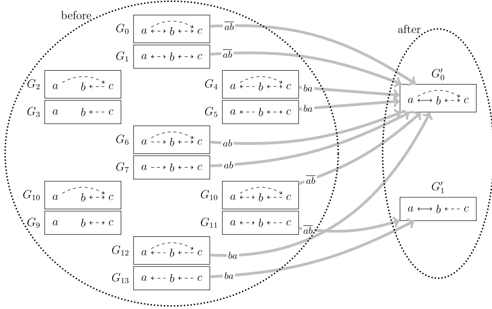
Fig. 1. Update of the indistinguishable gossip graphs for agent c after a call \bar{ab} .
