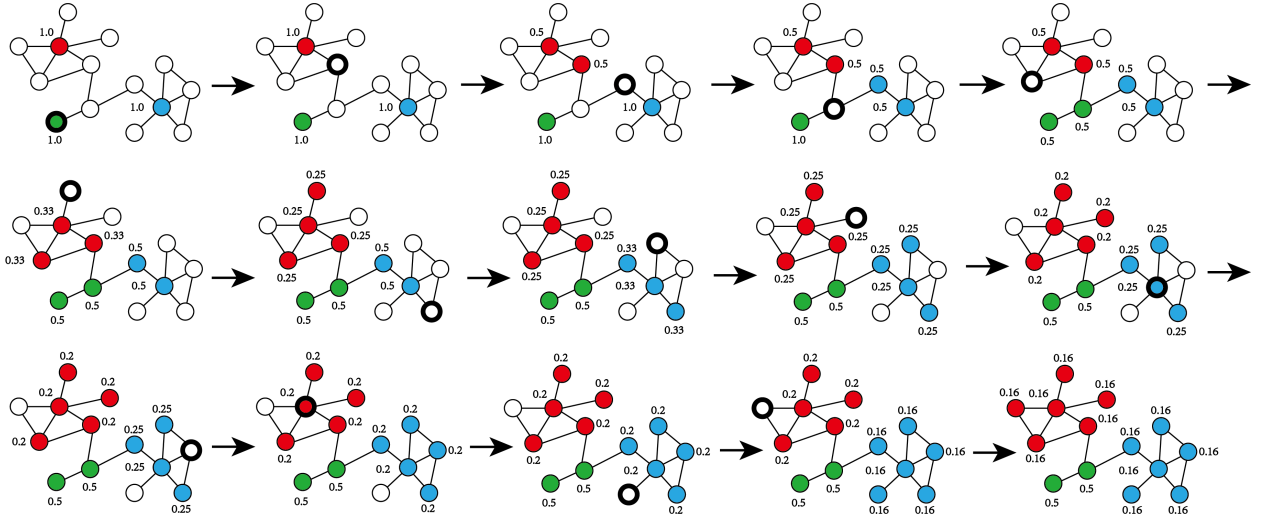
Figure 3: The workflow of FluidC for k_f = 3 communities (red, green and blue). Each node assigned to a community is labeled with the density of that community. The update rule is evaluated on each step for the node highlighted in black. Only the schematic results of the first iteration are given here.
