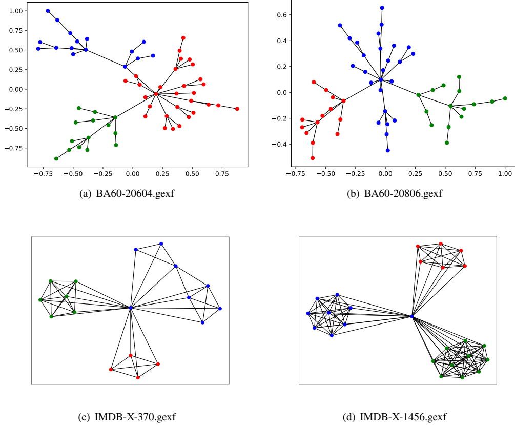
Figure 6: Examples of graph partition from BA-60 and IMDB-X datasets. Different colors represent different subgraphs.
