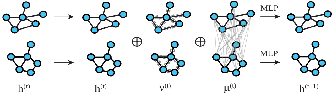
Figure 4: Propagation layer in node-level comparison. Each round of iteration is based on the embeddings of the previous round and the node-level comparison within each graph and between graphs.
