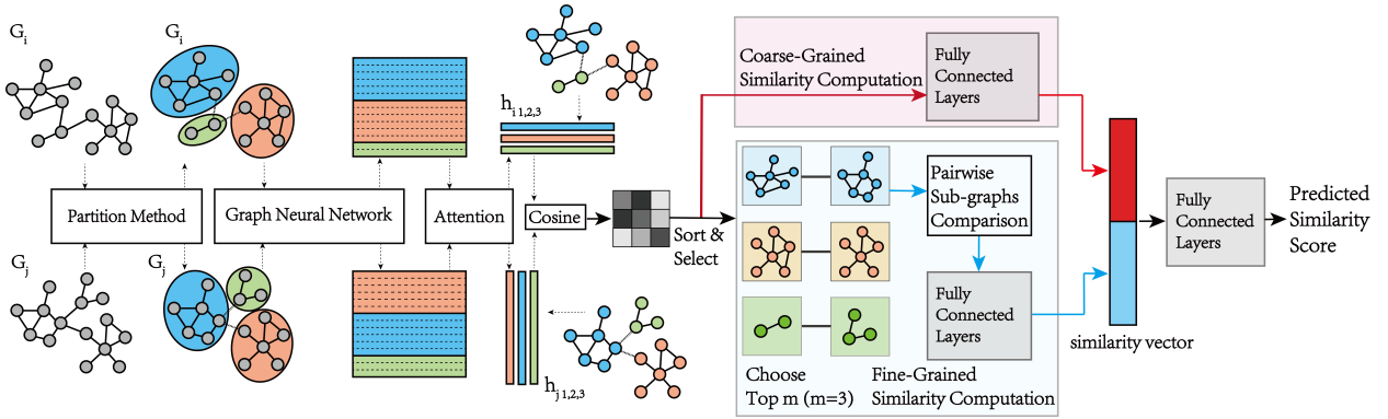
Figure 2: The general architecture of our model. The red arrows denote the data flow for subgraph-level interaction and the blue arrows denote the data flow for node-level comparison. After the graph partitioning method, only the top m (here m = 3 ) subgraph pairs with the highest similarity scores will conduct the node-level comparison.
