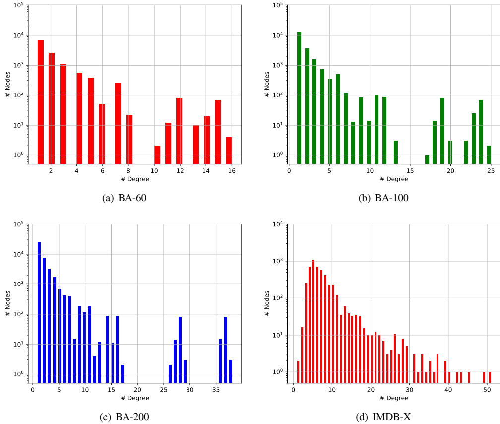
Figure 5: Nodes degree distribution of BA-model datasets.
