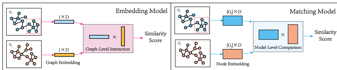
Figure 1: Two deep learning frameworks for graph similarity computation: embedding-model and matching-model. |G_i| and |G_j| represent the number of nodes of G_i and G_j , respectively, and D represents the embedding dimension. The red dashed box in G_i represents the subgraph of the G_i .
