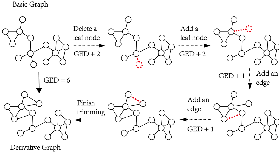
Figure 7: Generate a derivative graph with a GED of 6 from the basic graph. It is not necessary to use all three methods in real trimming. Here is only one case.
