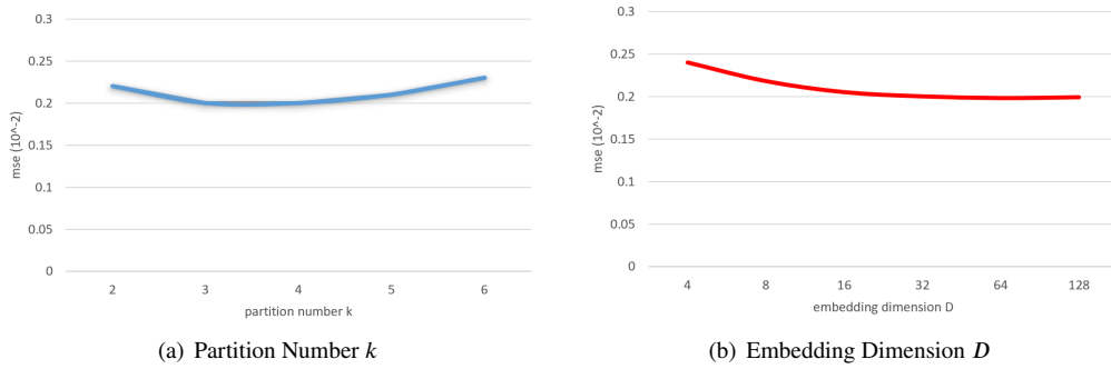
Figure 8: Mean squared error with respect to the partition number k and the dimensions D of subgraph-level embeddings.
