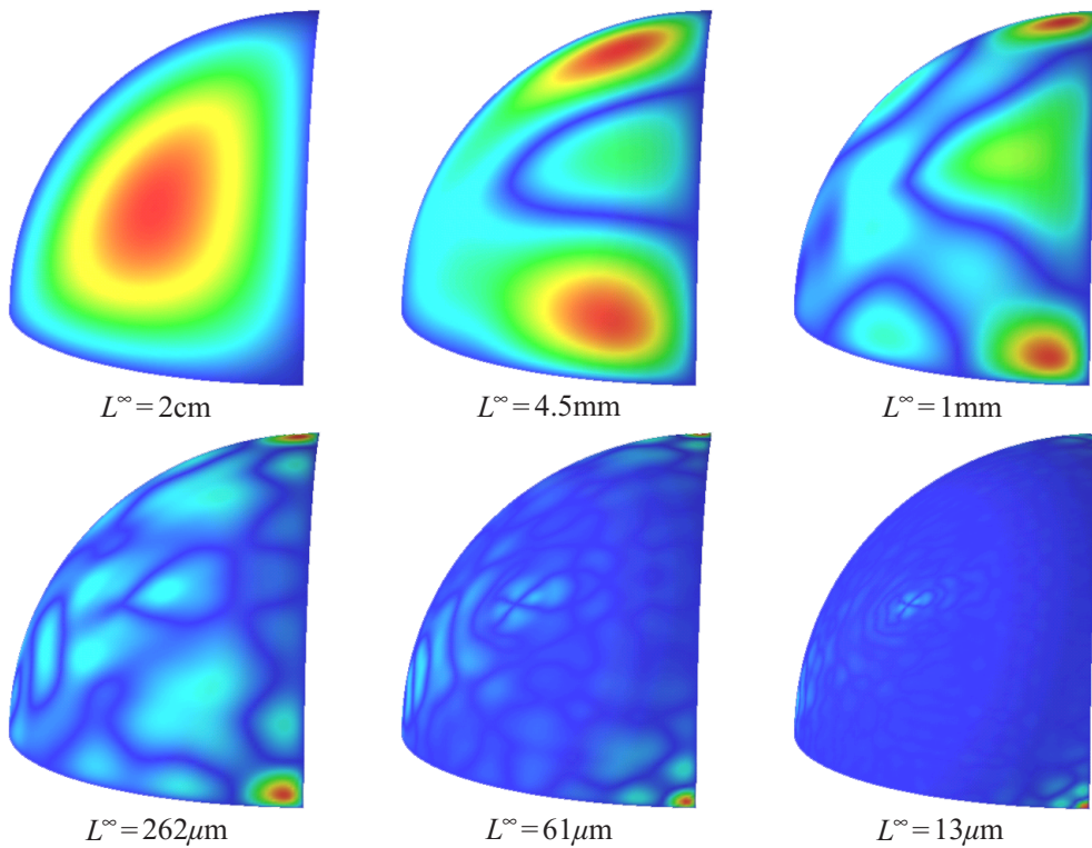
Fig. 7. Pseudo color images showing the successive approximation of the sphere octant by the combined subdivision surface with details computed through quasi-interpolation (Section 2.3).
