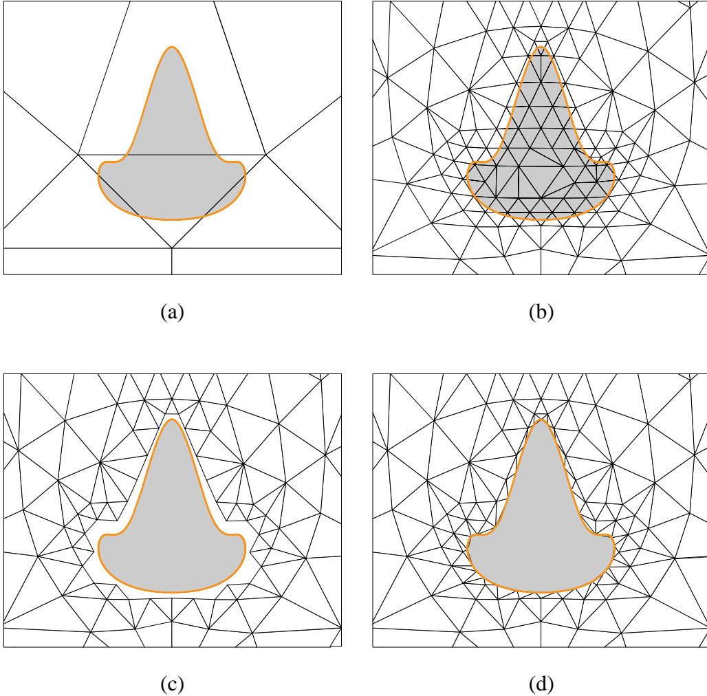
Fig. 9. (a) An initial non-symmetric combined subdivision surface with an approximate pre-image of the trim curve. (b) The triangles in the pre-image are refined as needed to adapt to the curve complexity. (c) Extraneous triangles are removed. (d) The curve is attached to the mesh. Subsequent relaxation optimizes the control point position and triangle quality. The result is the trimmed combined subdivision surface.
