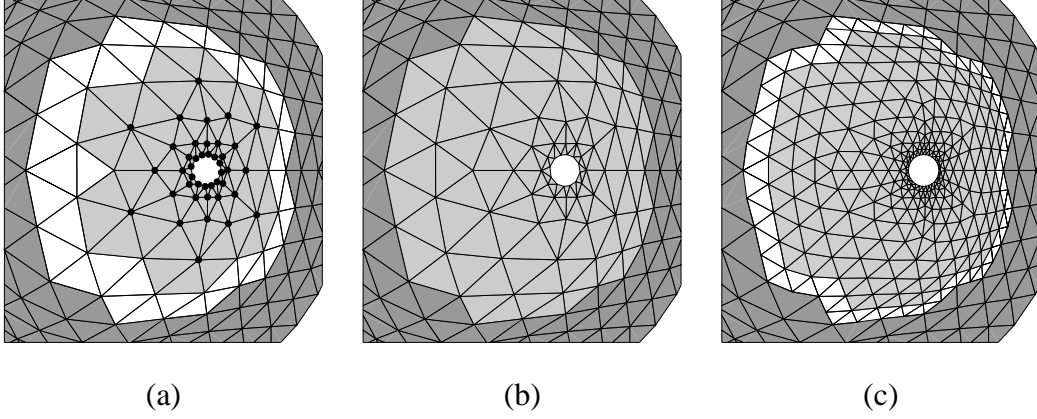
Fig. 11. (a) The input set T^0 is illustrated by the region shaded light gray, with the modified vertices marked. The limit surface corresponding to the dark shaded region matches the original surface exactly and must be preserved. (b) The limit patches that are compared to the original surface are given by N(T) . (c) The set T^1 is produced in the refinement step.
