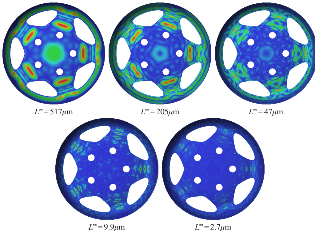
Fig. 13. Pseudo color images showing the error at successive levels of approximation. Shown top left is the surface generated by the remeshing algorithm, before detail coefficients were computed. The colors were rescaled for each pseudo color plot.
