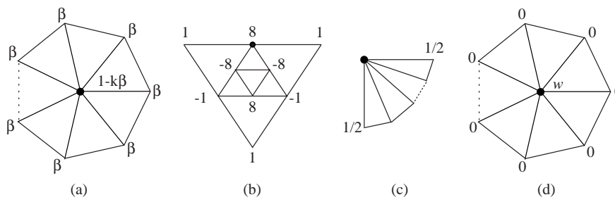
Fig. 5. Detail stencils for (a) interior, (b) boundary, (c) corner and (d) irregular vertices at levels j > 0 . For interior vertices, stencil (a) with \beta = -1/(2k) is quasi-interpolating and stencil (d) with w = (3 + \alpha)/3 (see Figure 2) is interpolating. Note that the corner stencil (c) is applied to detail vectors rather than differences.
