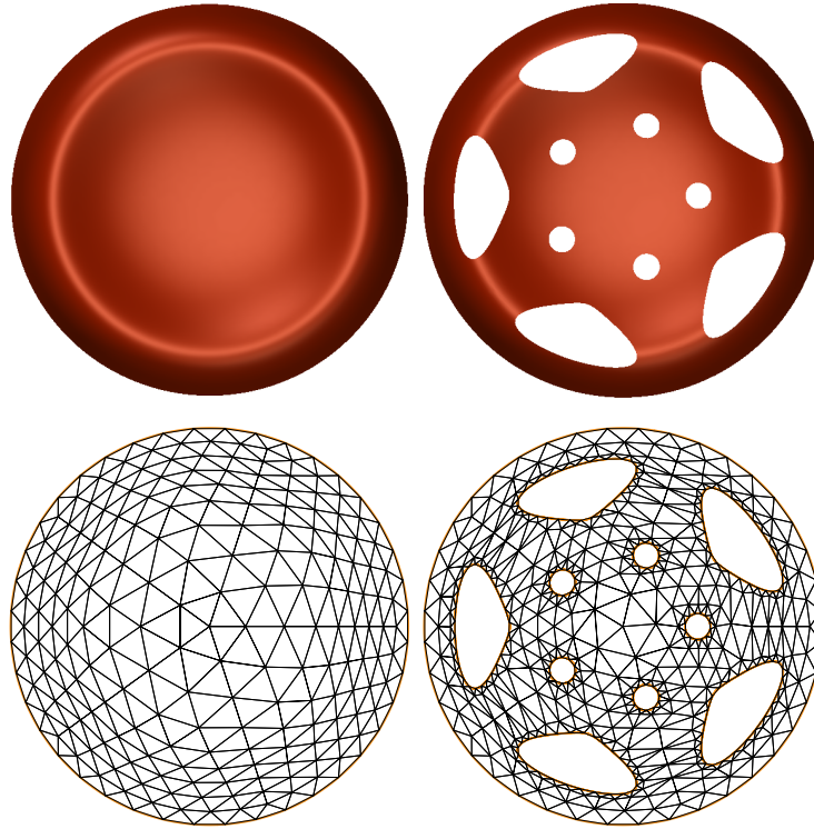
Fig. 12. The initial plate model (left) and the trimmed hubcap model (right). The corresponding control meshes are shown on the bottom.
