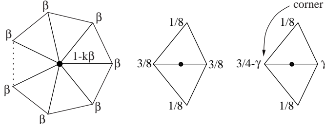
Fig. 2. Loop subdivision rules for the interior of surfaces. The rule for vertices, ordinary edges and edges adjacent to a corner (see the text for the weight \gamma ) are shown on the left, middle and right, respectively. In the vertex subdivision stencil, \beta = \alpha/(8k) , with \alpha = 5 - (3 + 2 \cos(2\pi/k))^2/8 and k the valence of the center vertex. The limit position stencil has the same form with \beta = \alpha/(k(3 + \alpha)) .
