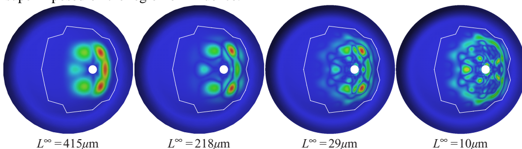
Fig. 14. Stages in the approximation of the original surface near a circular bore. The region of the control mesh affected by the remeshing algorithm is shown on the far left. To the right, the triangles being approximated at successive levels of refinement are shown superimposed on the region of influence.
