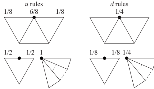
Fig. 3. At the boundary/corner ( u, d ) values are propagated to finer levels as indicated by these stencils.
