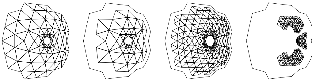
Fig. 14. Stages in the approximation of the original surface near a circular bore. The region of the control mesh affected by the remeshing algorithm is shown on the far left. To the right, the triangles being approximated at successive levels of refinement are shown superimposed on the region of influence.
