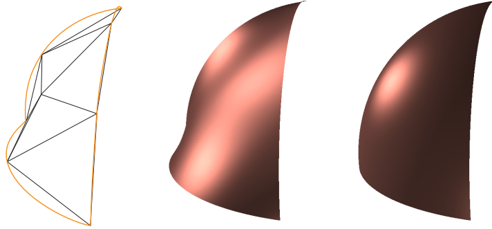
Fig. 6. Control mesh (left) and associated limit surface (middle). On the right the result of adding detail coefficients to ensure that the resulting surface matches an octant of a sphere.
