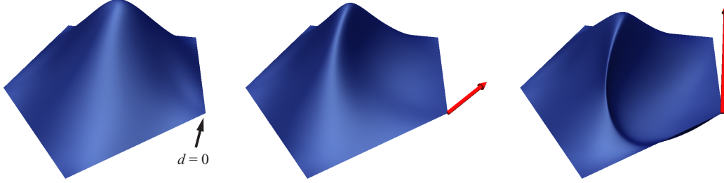
Fig. 4. Influence of the vector valued detail d at an exemplary boundary control point, illustrated by the red arrows. Note the influence on the surface shape near the boundary.
