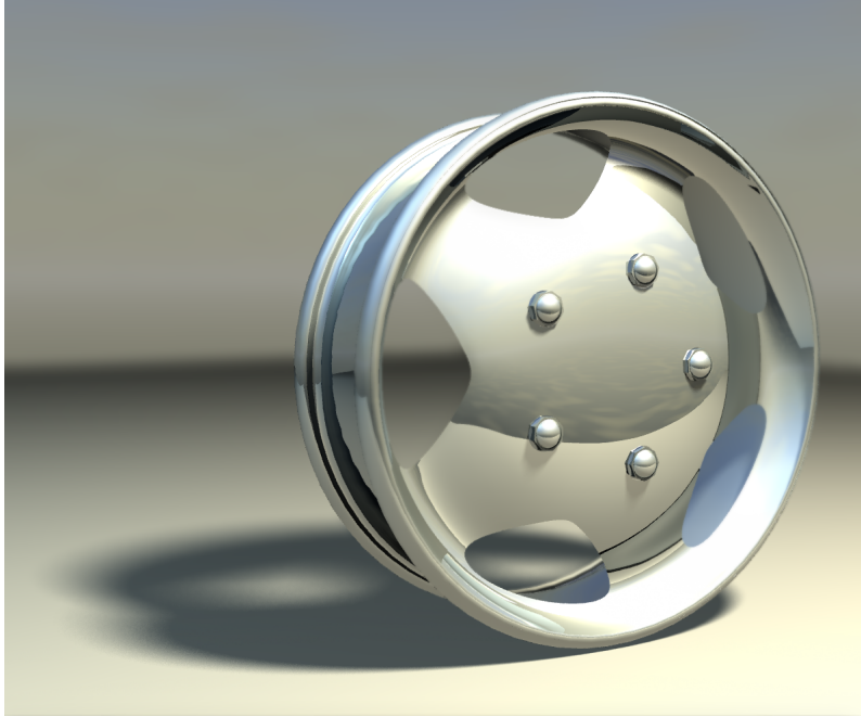
Fig. 1. Example of a subdivision surface after trimming with our procedure.
