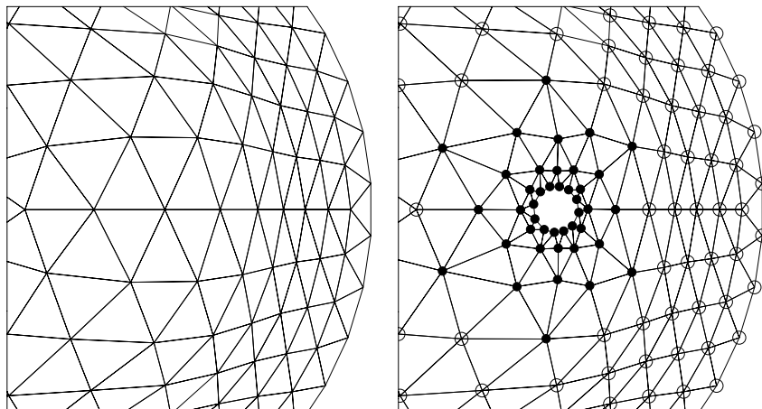
Fig. 10. The control mesh for the original surface (left) and the trimmed control mesh (right). The marked control points have their natural correspondence improved.
