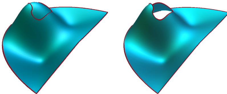
Fig. 8. The input to the trimming algorithm is a combined subdivision surface and a trim region on the surface (left). The trim region is removed and the trim curve is interpolated at the boundary of the surface (right).
