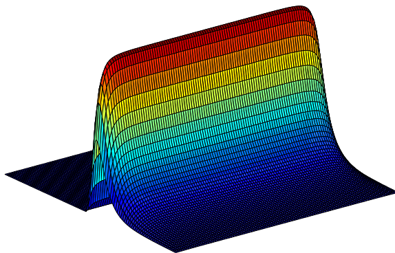
Figure 1: The journal bearing problem with \varepsilon = 0.9 .
