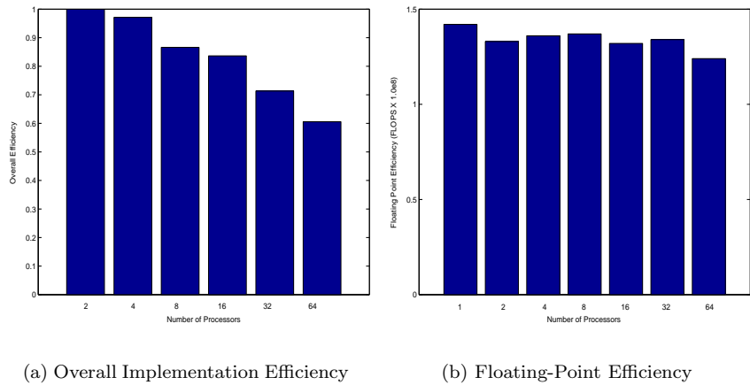
Figure 2: Parallel efficiency on the obstacle problem.
