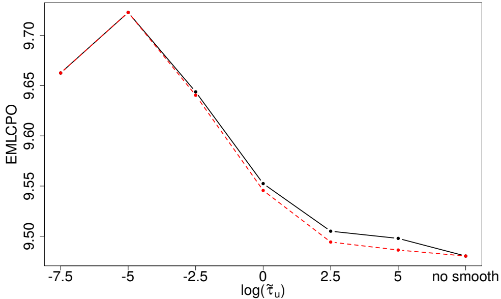
Figure 6: EMLCPO values for 6 different degrees of smoothness as well as no smoothing, the last being the results directly from Step 1. The dashed red indicates marginal posteriors computed with a point mass and the black solid with the Gauss-Hermite quadrature. From left to right: very smooth to no smoothing.
