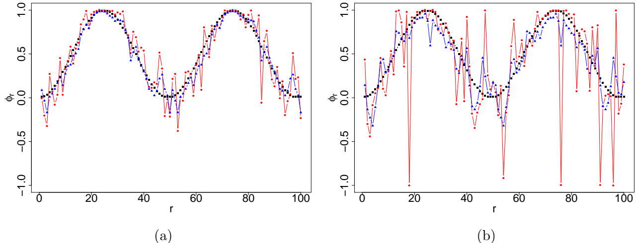
Figure 2: Values of \phi_r used to simulate R = 100 time series from (1) of length 50 (black squares), estimated values of \phi_r from fitting the AR(1) model to the simulated data (red circles), and estimates after fitting a smoothing spline (blue triangles). The left plot corresponds to simulations with fixed \tau = 2 and the right plot corresponds to \tau = 1 .
