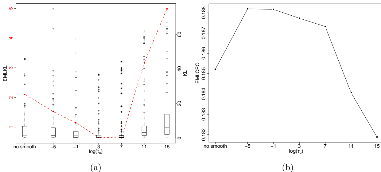
Figure 4: Comparison of inference and prediction performances between the standard non-smoothing method and the proposed smoothing approach from fitting (1). (a): EMLKL (dashed red, left y -axis) and KL_r (black, right y -axis) for no smoothing along with 6 different degrees of smoothness. Lower values of \log(\tau_u) indicate less smoothing. (b): Corresponding EMCPO for the same degrees of smoothing.
