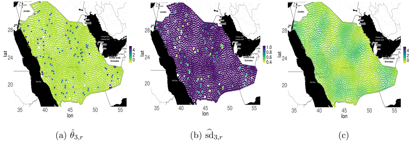
Figure 5: Map of the estimated (a) mode and (b) standard deviation of \tilde{\pi}(\theta_{3,r} \mid \mathbf{y}_r) for the R = 2000 regions shown in Figure 1b. (c) posterior mode of \tilde{\pi}_{\text{smooth}}(\theta_{3,r} \mid \mathbf{y}) .
