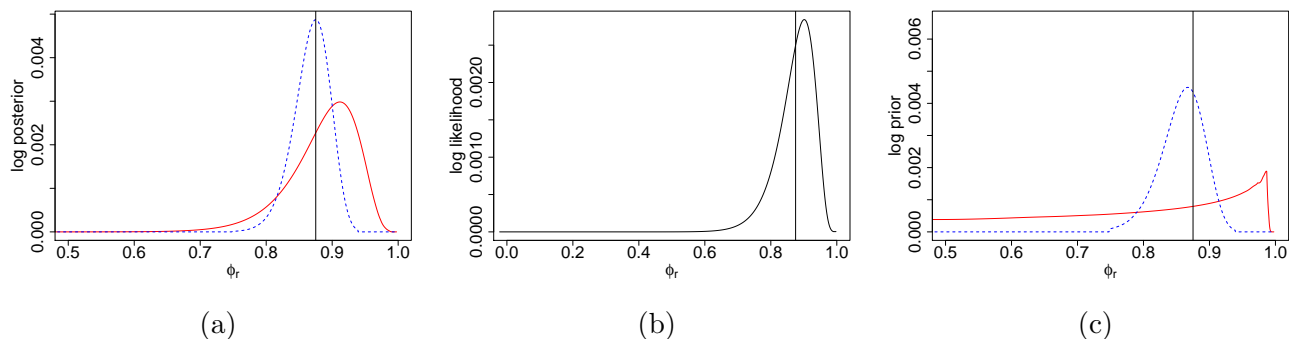
Figure 3: Comparison between non-smoothing and smoothing changes in the posterior distribution of \phi_r for the model (1). (a): Scaled log posterior distributions from Step 1 (solid red) and Step 2 (dashed blue). (b): Scaled log likelihood function. (c): Scaled log prior distributions from Step 1 (solid red) and Step 2 (dashed blue). The vertical line is the true value \phi_r = 0.88 .
