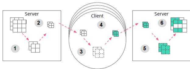
Fig. 6: The compression techniques considered are summarized above by the diagram from authors in [94]. (i) Federated dropout to reduce size of model (ii) Lossy compression of model (iii) Decompression for training (iv) Compression of participant updates (v) Decompression (vi) Global aggregation
