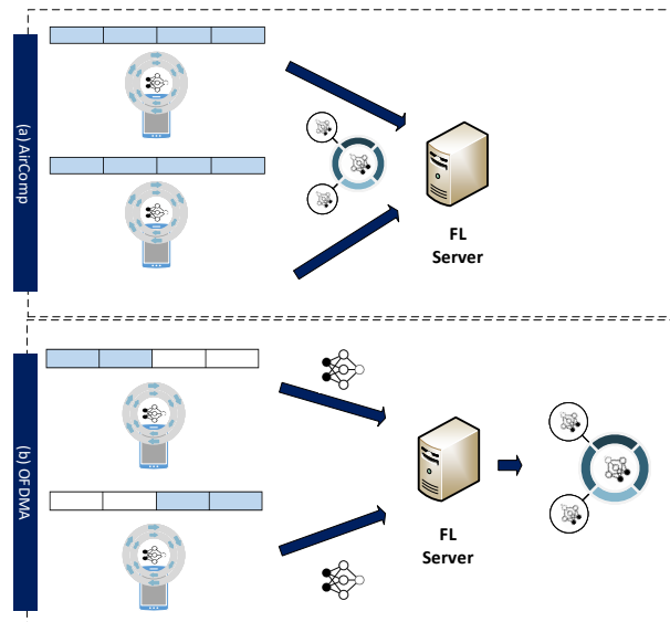
Fig. 8: A comparison [127] between (a) BAA by over-the-air computation which reuses bandwidth (above) and (b) OFDMA (below) which uses only the allocated bandwidth.
