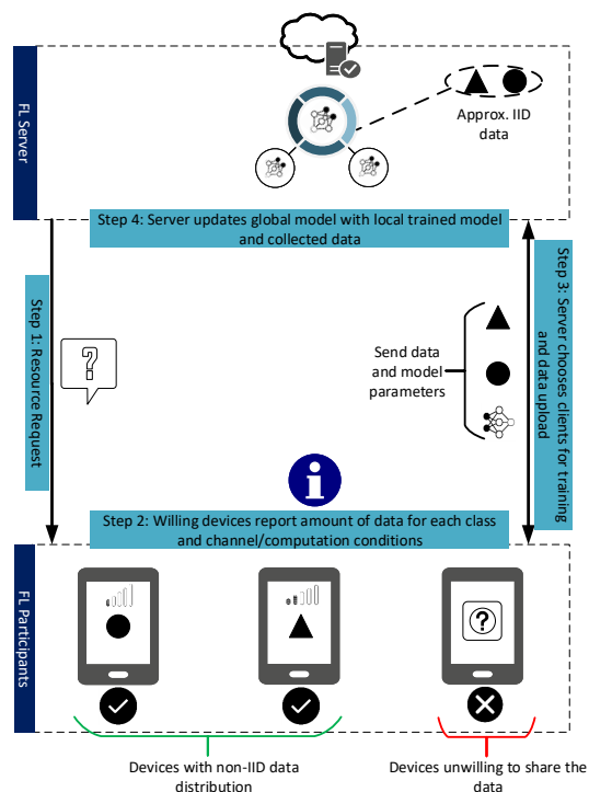
Fig. 7: Participant selection under FedCS and Hybrid-FL protocols.
