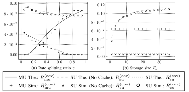
Figure 3: Evolution of average delivery rate in coverage-aided deployment. \lambda_{cr} = 1.0 \times 10^{-5} , \lambda_{mc} = 1.5 \times 10^{-5} , \lambda_{sc}' = 5.5 \times 10^{-5} , \lambda_{ut-m} = 12.8 \times 10^{-5} unit/m 2 ; P_{mc} = 16 , P_{sc} = 3 Watt; \tau_{mc} = \tau_{sc} = 4 bits/s/Hz; \alpha = 4 ; R_c = 80 meters; \mu = 30 bits/s/Hz; \gamma = 0.6 ; f_0 = 500 GByte; F_{sc} = 4 GByte; \eta = 1.45 .
