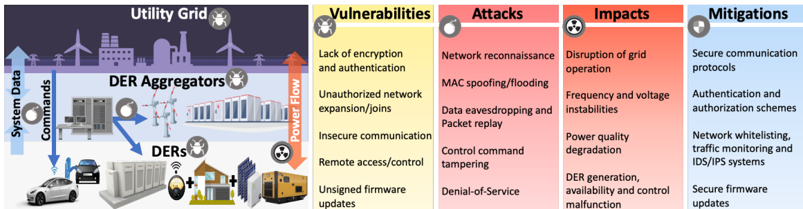
Fig. 6: Overview of DER-integrated electric grid that illustrates how the layered architecture expands the threat surface.
