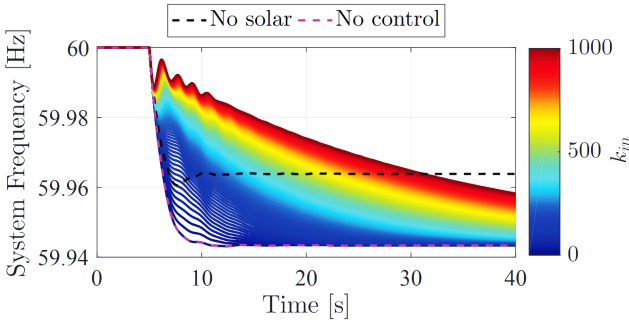
Fig. 3: Impact of synthetic inertia gain ( k_{in} ) on system frequency response [20].
