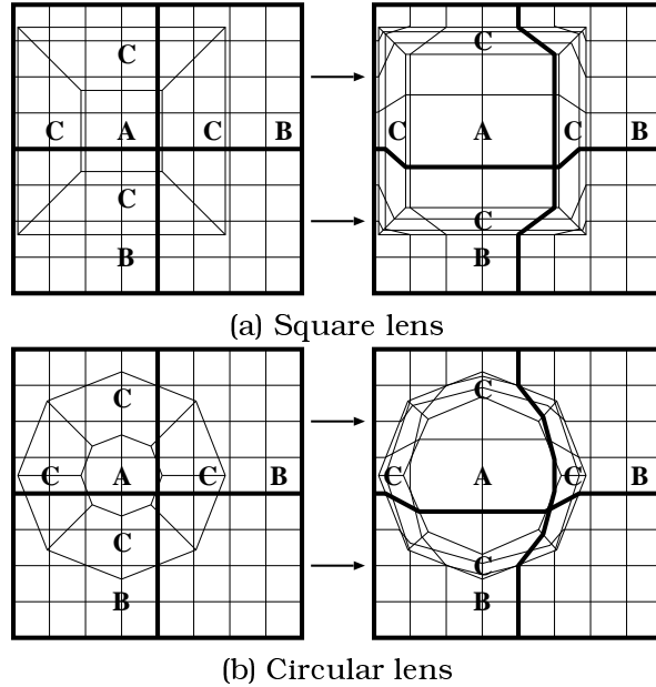
Figure 5. Local geometric transformations: Letters A-C denote separate transformations: A: Magnified, center region of the lens; B: Non-magnified, outer region; C: Warp-magnified region that blends the inner, magnified, region (A) to the outer, non-magnified, region (B).
