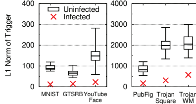
Fig. 4. L_1 norm of triggers for infected and uninfected labels in backdoor models. Box plot shows min/max and quartiles.
