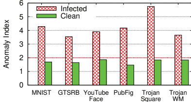
Fig. 3. Anomaly measurement of infected and clean model by how much the label with smallest trigger deviates from the remaining labels.
