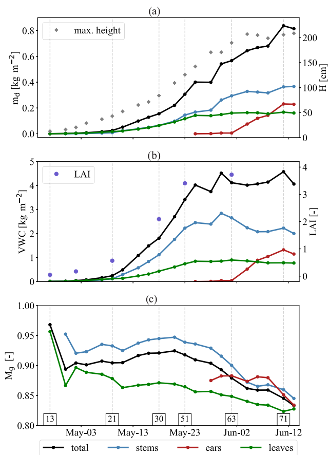
Fig. 2. Seasonal patterns of (a) dry biomass and maximum canopy height, (b) predawn VWC and LAI, and (c) predawn gravimetric water content, including the contributions of dominant plant constituents to total. Important phenological stages are represented by BBCH codes, which are explained in Table II.
