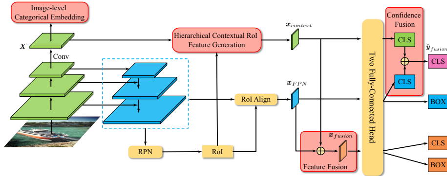
Figure 2. Overview of our Hierarchical Context Embedding (HCE) framework. At the image-level, we design an image-level categorical embedding module upon the detection backbone, which enables the network to learn object-level concepts from global-level context. At the instance-level, we generate hierarchical contextual RoI features that are complementary to conventional RoI features, and design the early-and-late fusion strategies ( i.e. , feature fusion and confidence fusion ) to make full use of the contextual RoI features for improving the classification accuracy of the detection head.
