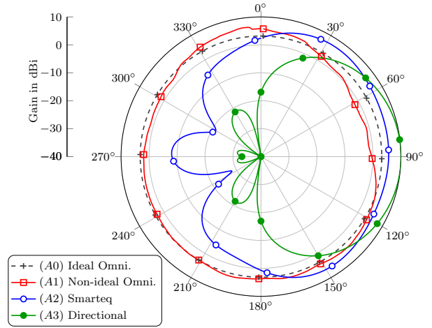
Fig. 3. Test antennas radiation patterns, |g(\phi)|^2 , in dBi. All antennas have the same average power gain in the azimuth plane. (Omni. i.e., Omnidirectional).
