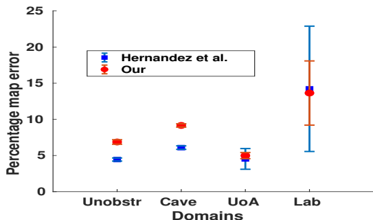
Fig. 14: Comparison of our strategy with the multi-robot mapping strategy in Hernández et al. [55]. The comparison is performed for the environments in Figure 4a, Figure 4b, Figure 4c, and Figure 4d. For each environment, the dot and square represent the median of the maximum error in the maps produced by our strategy and by the one in [55], respectively, over 10 simulation trials. The corresponding error bars indicate the largest and smallest maximum errors over the trials.
