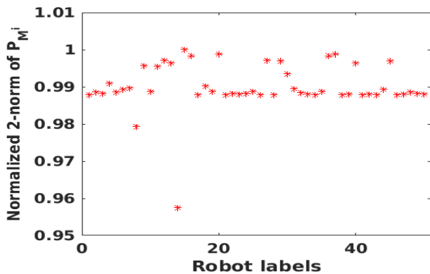
Fig. 9: Consensus over maps. The metric \|\mathbf{P}_{M^i}\|_2/\max_i\|\mathbf{P}_{M^i}\|_2 , where \mathbf{P}_{M^i} is the set \bar{\mathbf{P}}_{M^i} in matrix form, for each robot R^i in a swarm of 50 robots that explore the environment in Figure 4e for t_f = 3600 s.
