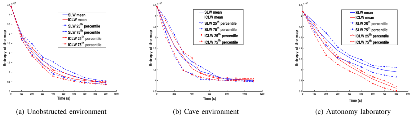
Fig. 12: Time evolution of the entropy H(M^i) , computed using Equation (1), of occupancy maps M^i , i = 1, \dots, N_R , from simulations of: (a) N_R = 5 robots mapping the unobstructed environment in Figure 4a; (b) N_R = 5 robots mapping the cave environment in Figure 4b; and (c) N_R = 20 robots mapping the autonomy laboratory in Figure 4d. For each environment, 30 simulation trials were run in which the robots performed a standard Lévy walk (SLW), and 30 trials were run in which they performed the information correlated Lévy walk (ICLW) presented in Section III. The following plots are shown in each subfigure: mean entropy over 30 trials with the SLW (solid blue lines); mean entropy over 30 trials with the ICLW (solid red lines); 25 th percentile of the 30 trials with the SLW (blue dashed lines with circles); 75 th percentile of the 30 trials with the SLW (blue dashed lines with squares); 25 th percentile of the 30 trials with the ICLW (red dashed lines with circles); 75 th percentile of the 30 trials with the ICLW (red dashed lines with squares).
