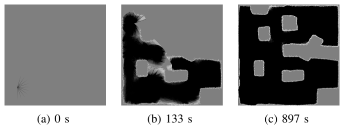
Fig. 7: The occupancy grid map generated by the robot inside the green dotted circle in the snapshots in Figure 6 at the times of these snapshots.
