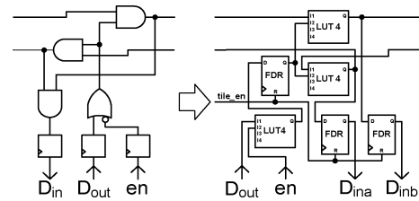
Fig. 8. Xilinx Virtex-4 implementation of a bidirectional multipoint connection in the embedded macro.
