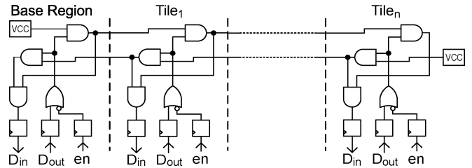
Fig. 7. 1-Bit bidirectional multipoint connection in the embedded macro.
