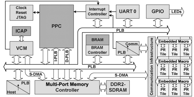
Fig. 14. Overview of the system implementation.
