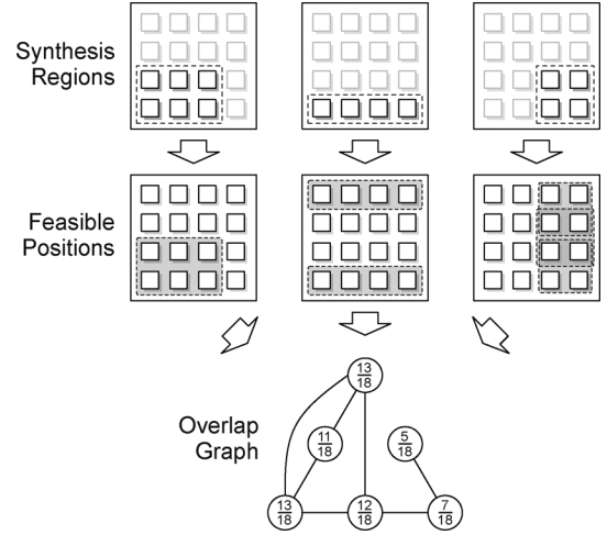
Fig. 13. Design steps from the selection of the synthesis region to the computation of the overlap weight considering only one PR module for each dynamic system component.
