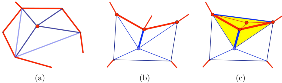
Figure 4: A wheel with a central hub (a). Given two non-adjacent rim vertices on different paths (b), there is no edge connecting them provided the boundary of the disc is clean. (c) gives a boundary which is not clean.
