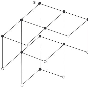
FIGURE 1. A DAG where 2 greens are needed to win. The white nodes are the sinks.
