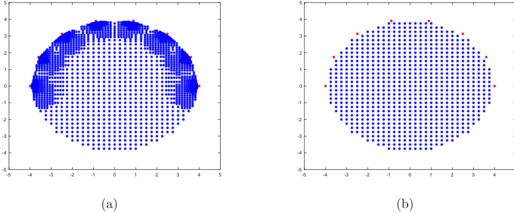
Figure 6: (a) Grid points with mesh-size satisfying h_{z,v}(0.1) along the direction v , where v = (1, 0) and v = (0, 1) , respectively. (b) Unrefined mesh. Measurement points in red and grid points in blue.
