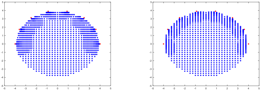
Figure 5: Grid points with mesh-size satisfying h_{z,v}(0.1) along the direction v , where v = (1, 0) and v = (0, 1) , respectively.
