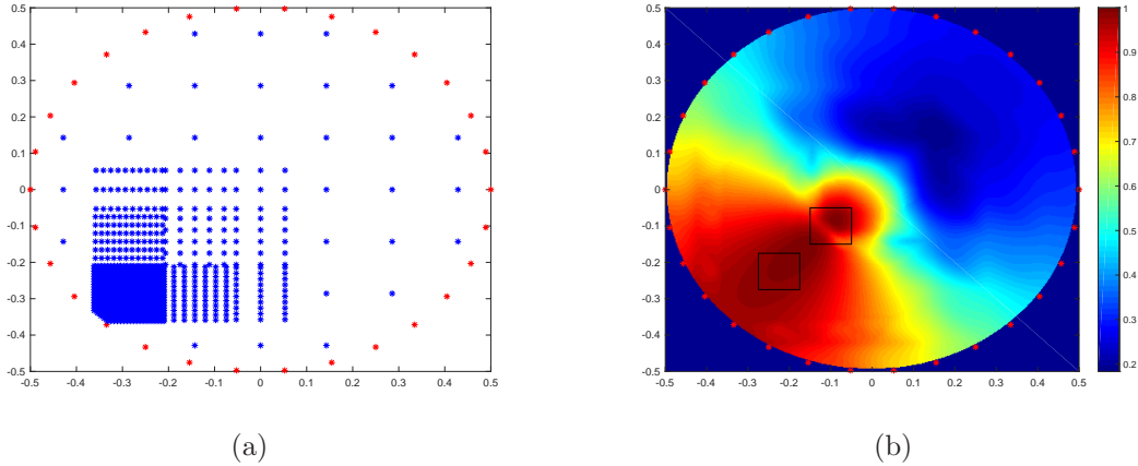
Figure 9: (a) Grid points on adaptively-refined mesh given by a tensor grid with mesh-sizes \widetilde{h_{x,e_i}}(\alpha) along e_1 = (1, 0), e_2 = (0, 1) , \alpha = 0.9 , and x is taken only when I_{\text{coarse}}(x) > 0.995 . (b) A reconstruction given by [I(x, dy)]^2 , where I(x, dy) in (2.12) with adaptively-refined grid on the left.
