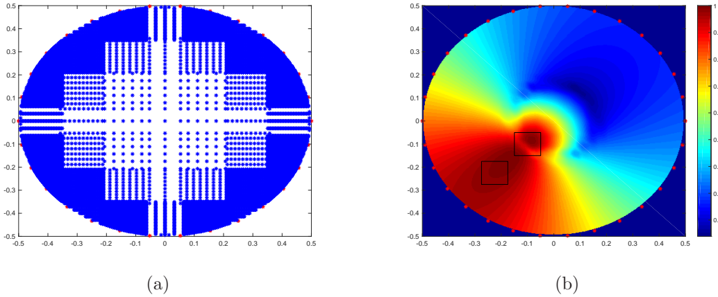
Figure 8: (a) Grid points on a refined mesh given by a tensor grid with mesh-sizes \widetilde{h}_{z, e_i}(\alpha) along e_1 = (1, 0) , e_2 = (0, 1) , \alpha = 0.9 , and x is taken in the whole sampling domain \Omega . (b) A reconstruction given by [I(x, dy)]^2 , where I(x, dy) in (2.12) with a refined grid in the left.
