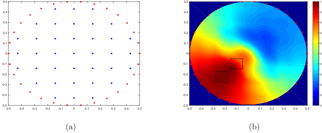
Figure 7: (a) Grid points on a coarse mesh. (b) reconstruction given by [I(x, dy)]^2 , where I_{\text{coarse}} := I(x, dy) in (2.12) with the grid point given by the coarse mesh.
