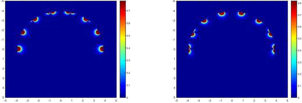
Figure 4: The function p_{v,\alpha}(z) at v = (1, 0) and v = (0, 1) , respectively, when \alpha = 0.99 . Measurement points in red and grid points in blue.
