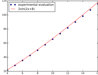
Figure 3: Average Stopping Time Approximation
