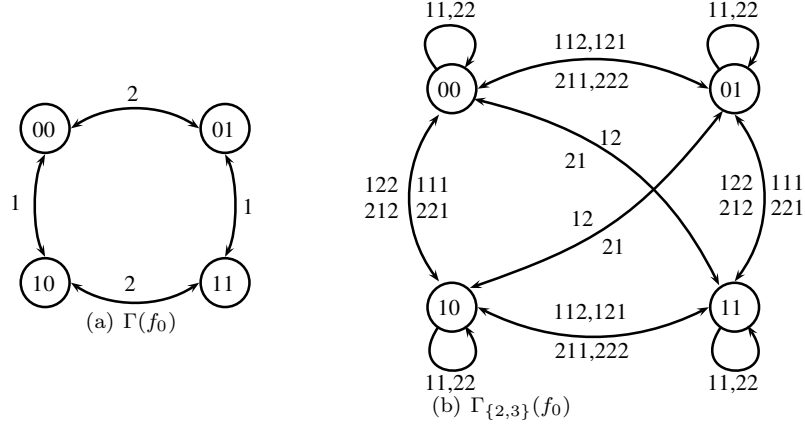
Figure 2: Iterating f_0 : (x_1, x_2) \mapsto (\overline{x_1}, \overline{x_2})
