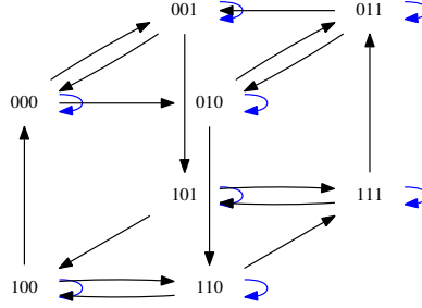
Figure 1: Iteration Graph \Gamma(f^*) of the function f^*
