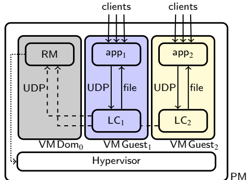
Figure 2: Architecture of a single Physical Machine (PM).
