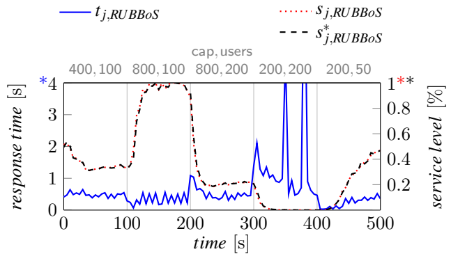
Figure 5: Controlling RUBBoS when both the cap and the number of users vary, p_1 = 0.9 , setpoint 0.5 seconds.
