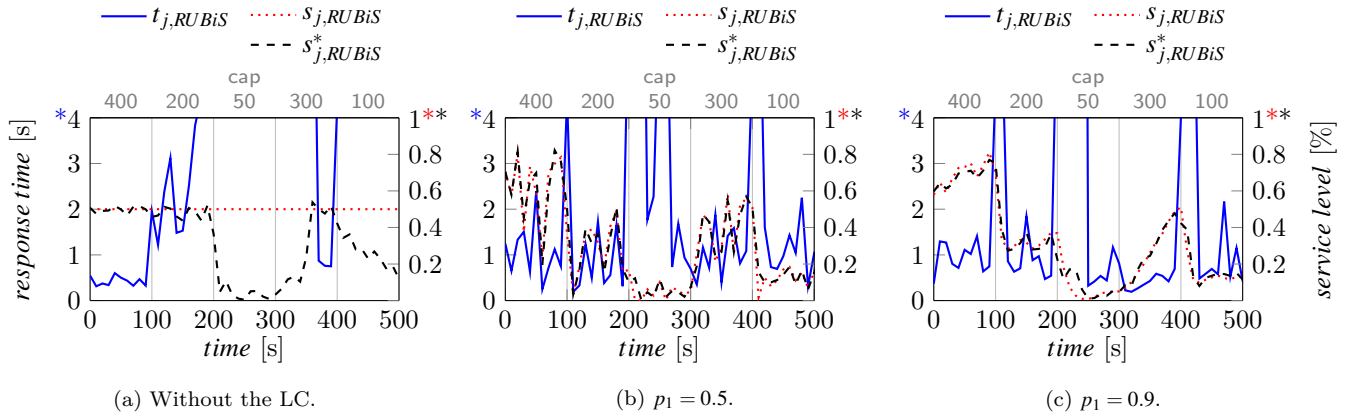
(a) Without the LC. (b) p_1 = 0.5 . (c) p_1 = 0.9 . Figure 3: Response time and probability of executing the recommender system varying the VM cap.
