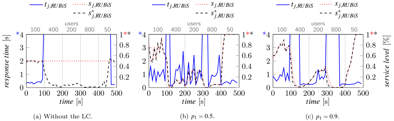
Figure 4: Response time and probability of executing the recommender system varying the number of users.
