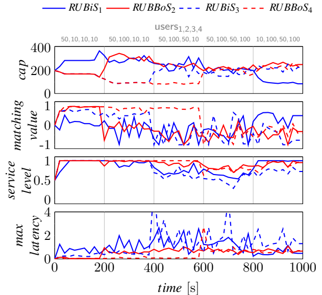
Figure 7: Resource manager and four applications.
