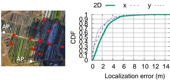
Figure 11: 2D accuracy with deployment in farm.
