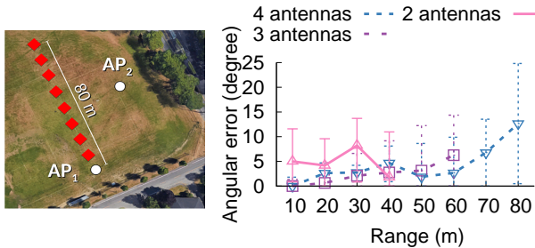
Figure 9: Stationary self-localization angular accuracy.
