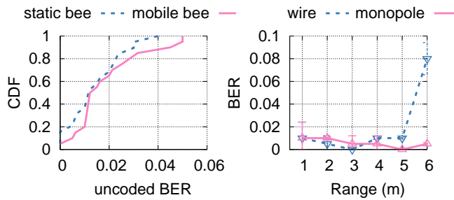
Figure 14: Backscatter performance. The unencoded BER is low and comparable to prior backscatter designs [77] and the bee can upload data when it is back at the hive.
