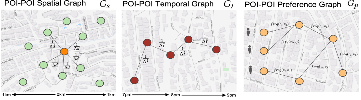
Figure 3: Illustration of how global spatial, temporal and preference factors are represented into POI-POI graphs. Maps © OpenStreetMap contributors, CC BY-SA.
