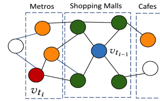
Figure 4: Input previous POI of v_{t-1} (blue vertex) and next POI of v_t (red vertex). Green vertices are first-order neighbours and orange vertices are higher-order neighbours found with random walks.
