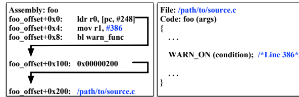
(b) Warning information: line number (i.e., 386) is the operand of assembly code; file name (i.e., /path/to/source.c ) is a constant string.
