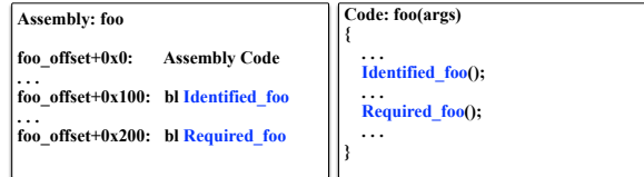
(c) Sibling relationship: Required_foo and Identified_foo are both called by foo
