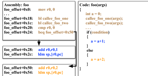
(b) Callee Number: The two callee functions (i.e., callee_foo_one, callee_foo_two) map to the two bl instruction at offset foo_offset+0x18 and foo_offset+0x1c. Basic Block Number: The three basic blocks in source code maps to three basic blocks in assembly code.
