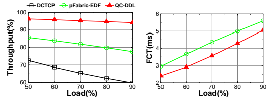
Figure 16: Deadline-Aware Scheduling on W4.
