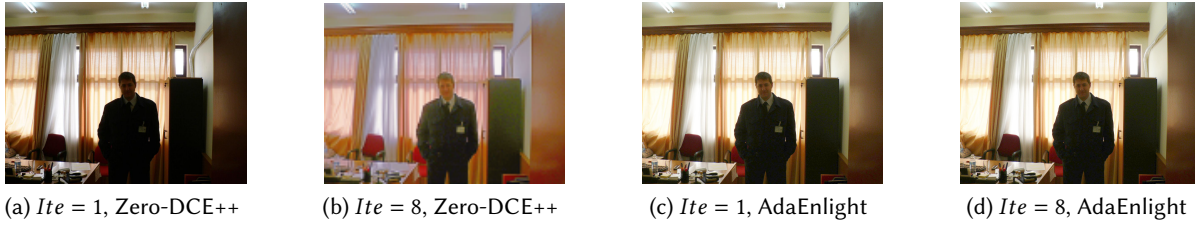
Fig. 17. Impact of iteration numbers Ite on visual quality by Zero-DCE++ and our Gamma correction-based curve.
