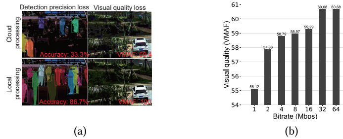
Fig. 3. Comparison of video enhancement locally on-device and remotely on-cloud. (a) Example frames enhanced by local processing and remote processing. The upper row follows the encode-decode-enhance pipeline of remote processing, while the lower row are directly enhanced as in local processing. (b) Enhanced video quality of the encode-decode-enhance pipeline under different frame bitrates into the video codec.
