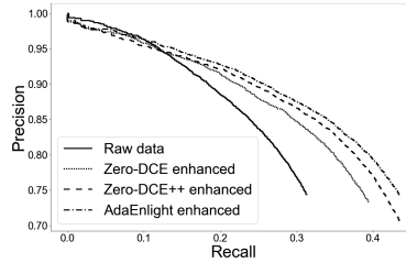
Fig. 13. Performance comparison for the downstream on-device video application of mobile face detection.
