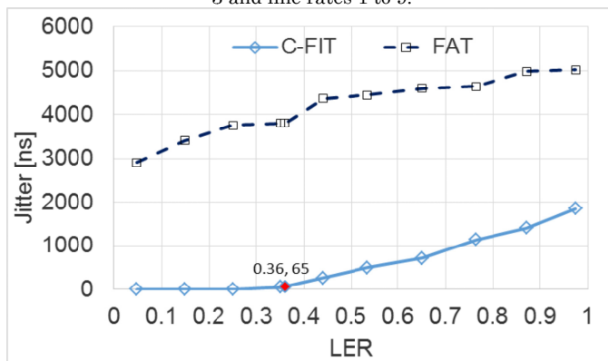
Figure 12: Jitter vs. Load to Ethernet Ratio for number of flows 4 to 6 and line rates 1 to 9.
