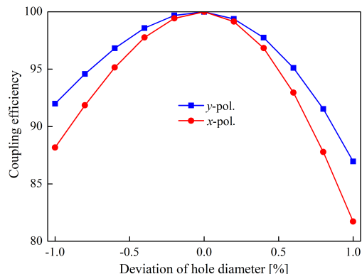
Fig. 11 Coupling efficiency for each polarization versus the deviation of all the air holes at same level.
