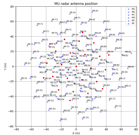
Fig. 8 Virtual receive sub-array positions for adaptive beamforming. The red points indicate the physical centers of the sub-array antennas, whereas the blue dots indicate those of the virtual sub-array antennas. The blue dots have transparency. The darker colors indicate overlapping antenna positions.
