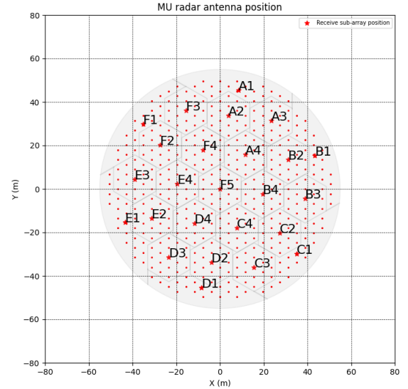
Fig. 6 Receive antenna positions. Star markers denote the receive antenna phase centers.
