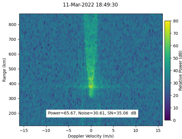
Fig. 12 Same as Fig. 11 except that the DDMA-MIMO processing was performed.
