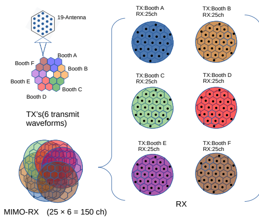
Fig. 3 Layout images of the actual transmit antenna (upper left), receive antenna (right), and virtual receive antenna (lower left).
