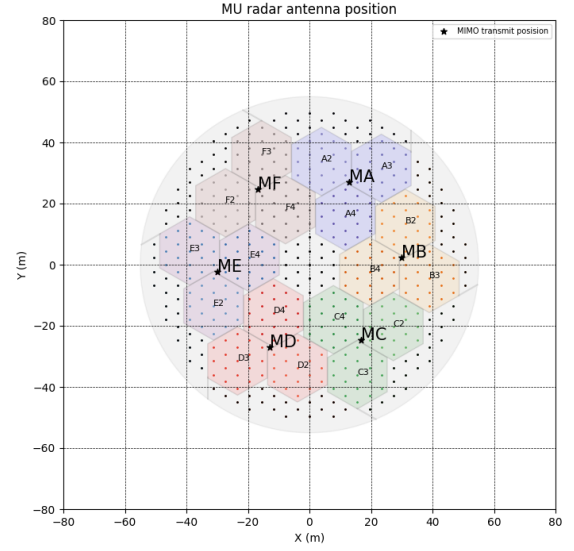
Fig. 5 Transmit antenna positions. Transmit antennas are divided into six groups of sub-array antennas (composed of 57 antenna elements) corresponding to the each booth (booth A (A2/A3/A4 in blue); B (B2/B3/B4 in orange); C (C2/C3/C4 in green); D (D2/D3/D4 in red); E (E2/E3/E4 in purple) and F (F2/F3/F4 in brown)). Star markers denote the transmit antenna phase centers, and the black points are not used for transmission.
