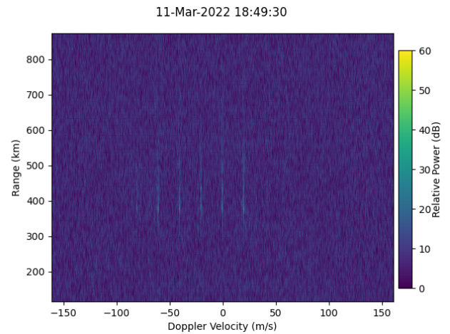
Fig. 10 Doppler spectra at A2 sub-array receivers observed at 1849 JST on 11 Mar 2022 before executing MIMO-processing. The horizontal and vertical axes show the target Doppler velocity and range with offset of 395 726 km due to echoes from 265 trips, respectively. Six receive signals derived from each orthogonal transmitter with DDMA-MIMO frequency offset (TX5, TX4, TX3, TX2, TX1, and TX6 from the left) were observed.
