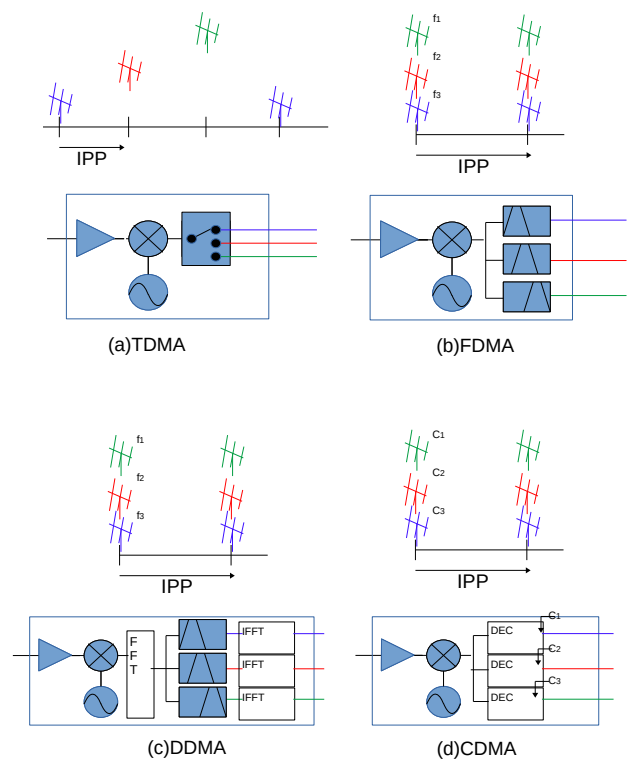
Fig. 2 Comparison between orthogonal waveforms (Configuration image).
