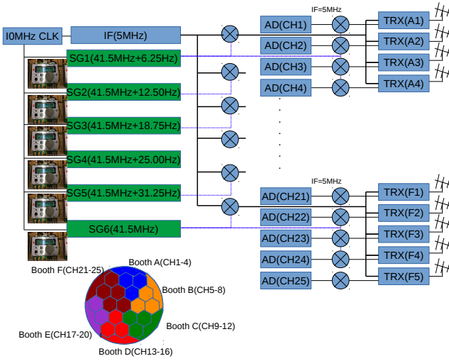
Fig. 4 DDMA-MIMO configuration of the MU radar. The green mark indicates additional settings, and the six orthogonal signals are distributed to the transmitters.
