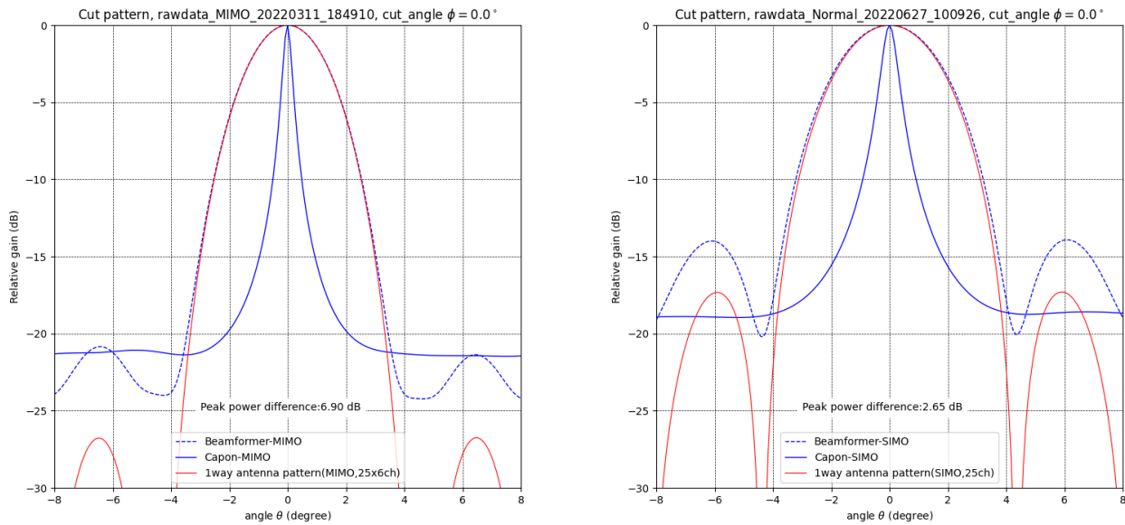
Fig. 16 Cut pattern at an azimuth angle of \phi = 0^\circ : Comparison between the beamformer, Capon, and calculated 1-way antenna pattern using MIMO (left) and SIMO (right) observations. The blue dotted and blue solid lines represent the angular distributions using the beamformer and Capon imaging, respectively, whereas the red line represents the calculated antenna pattern.
