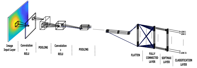
Fig. 3: Deep Learning Convolutional Neural Network architecture.
