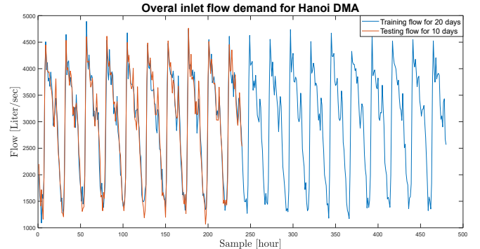
Fig. 5: Training and testing flow patterns.
