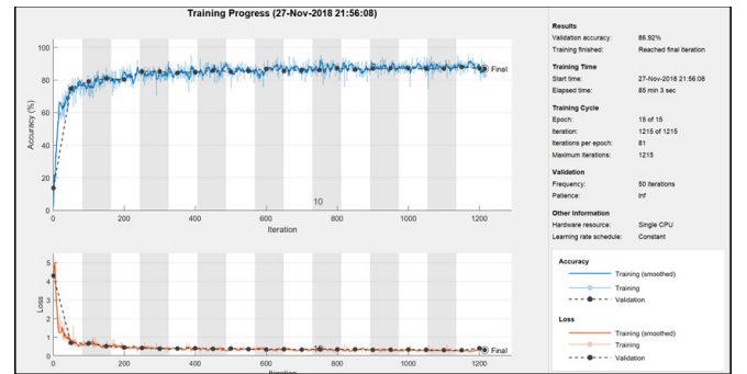
Fig. 7: CNN training process for the sensor configuration 7 (12 sensors) using the Deep Learning Toolbox TM of MATLAB ® .
