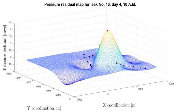
Fig. 6: A sample of pressure residual map.
