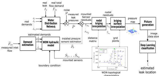
Fig. 1: Leak localization scheme using Deep Learning.
