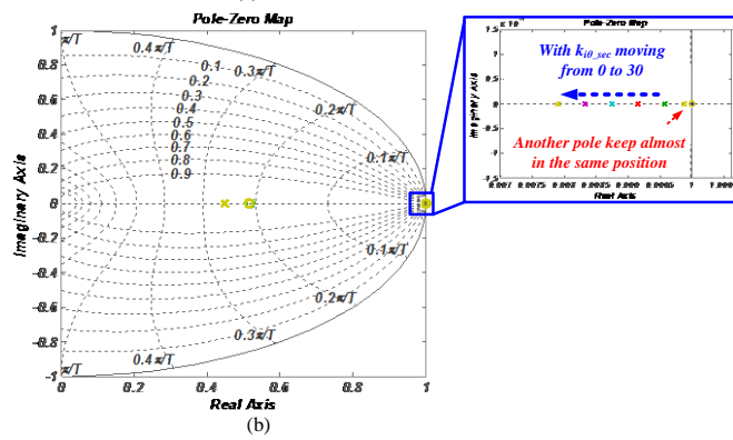
Fig. 13. pole-zero map for phase restoration. (a) PZ map with variable k_{pb\_sec} . (b) PZ map with variable k_{it\_sec} .
