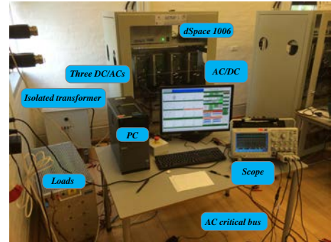
Fig. 15. Experimental setup.
