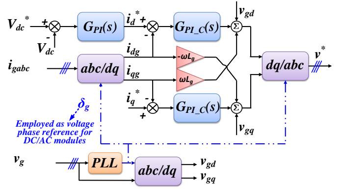
Fig. 2. Control diagram for AC/DC.
