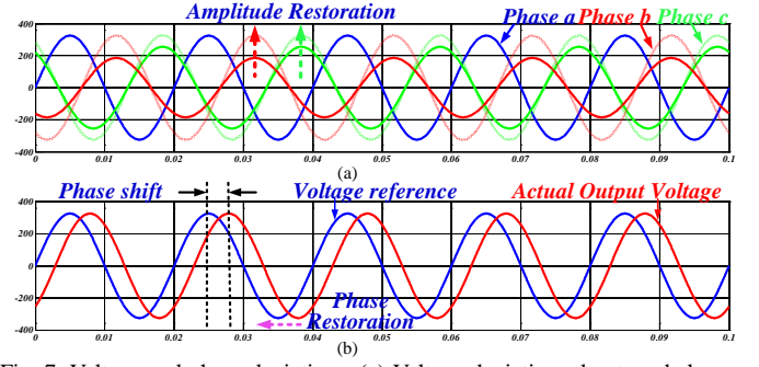
Fig. 7. Voltage and phase deviations. (a) Voltage deviations due to unbalanced load. (b) Phase deviations due to “reactive power-to-phase droop” or Q-\phi droop.
