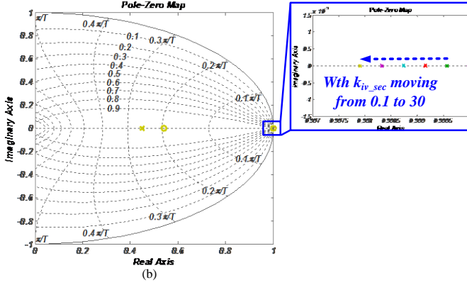
Fig. 12. pole-zero map of voltage amplitude restoration. (a) pz map with variable k_{pv\_sec} . (b) pz map with variable k_{iv\_sec} .
