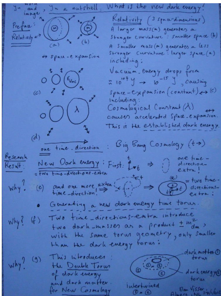
Fig. 1: The new dark energy is a Double Torus geometry existing of a dark energy torus and dark matter torus (intertwined) defined by three time-directions (two more than in Big Bang Cosmology) .
