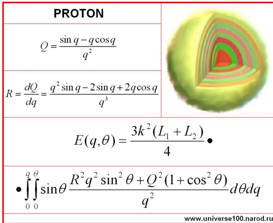
Figure 8. Portrait of proton.
