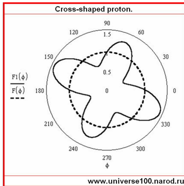
Figure 9. Any possible section of proton if L_1 \ll L_2 .
