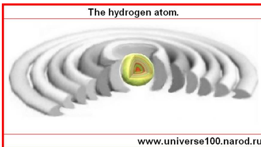
Figure 10. Portrait of hydrogen.
