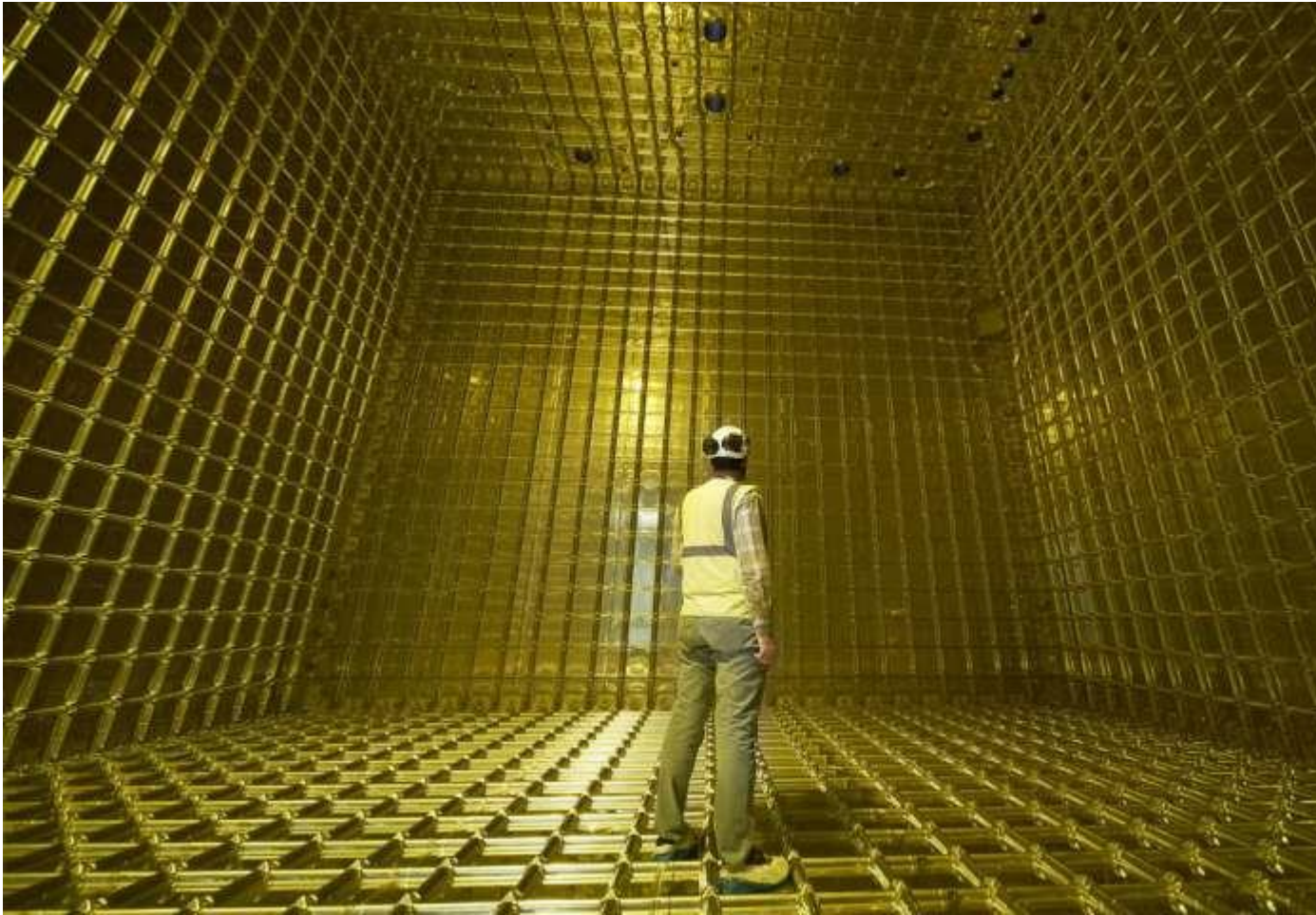
Inside the first ProtoDUNE detector, before it was filled with liquid argon. Credit: CERN
