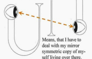
Figure 16, Anti matter deficit problem solved by mirror symmetric undivided ( entangled ) Multiverse without dead or alive Cats in boxes.
