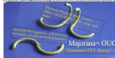
Figure 12, particle schemes of Quantum FFF Theory.
