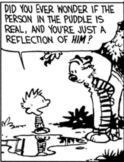
Figure 16, Anti matter deficit problem solved by mirror symmetric undivided ( entangled ) Multiverse without dead or alive Cats in boxes.
