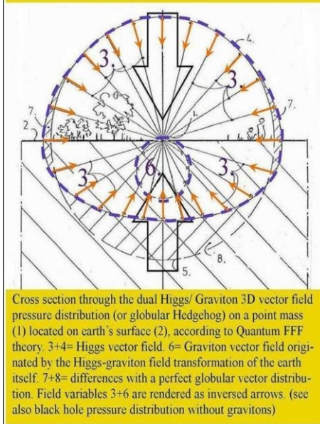
Figure 15, Quantum gravity.
