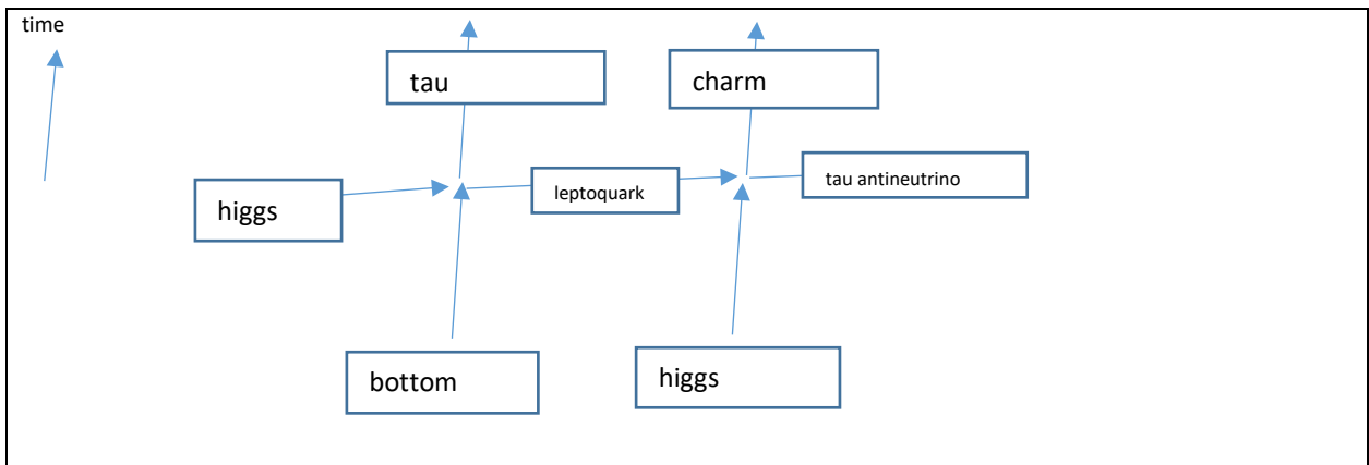
Figure 2B Leptoquark exchange between b \tau and c \nu'
