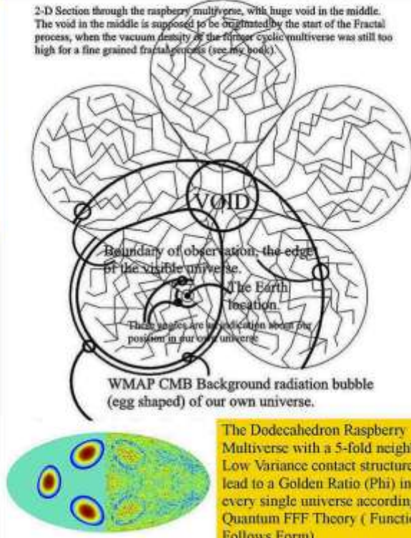
Figure 5, wavefunction collapse between CP symmetric mirror particles by instant entanglement between multi universal bubbles located around the Big Bang central void.
