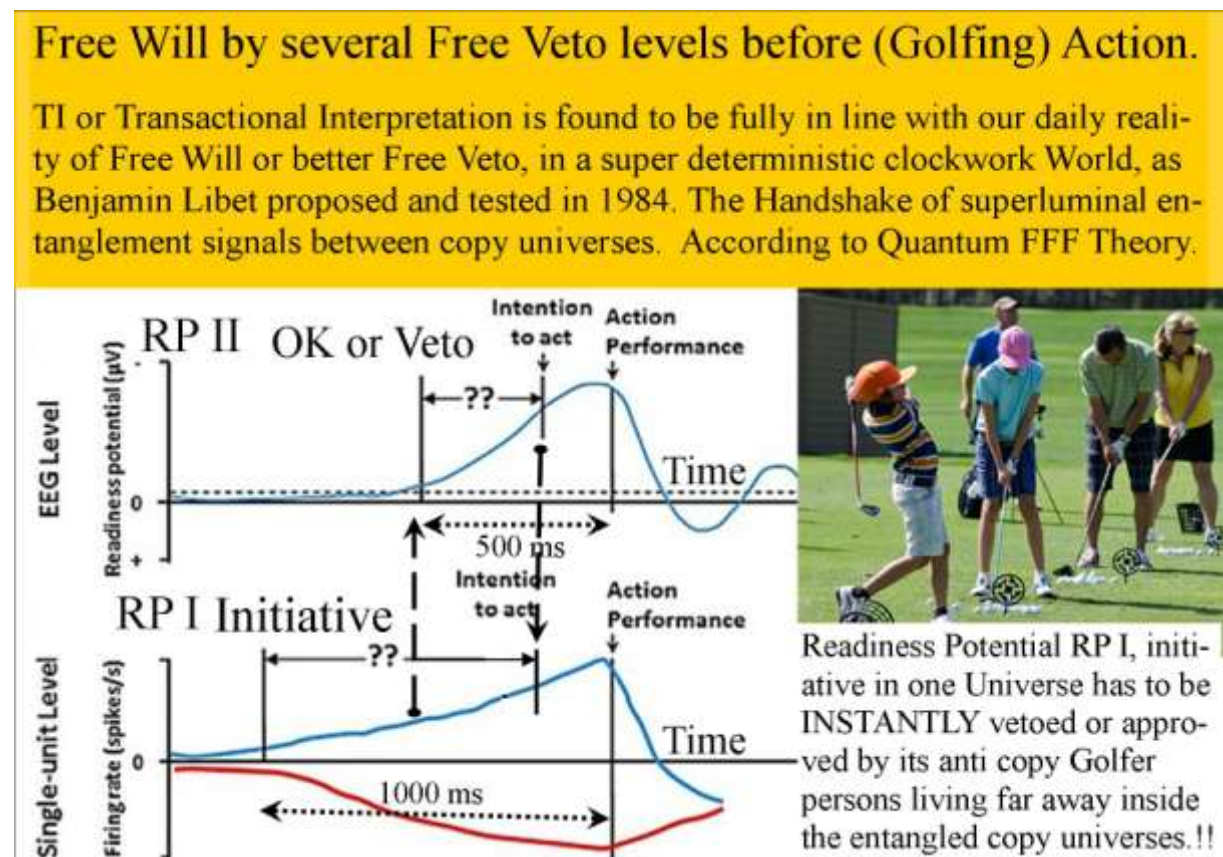
Figure 1, TI and several Veto handshake levels before hitting a golf ball.
