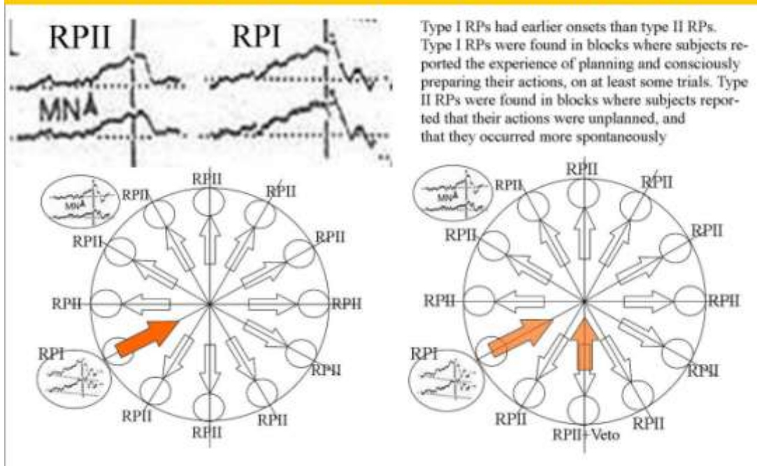
Figure 10, Quantum FFF Theory explanation of the difference between RPI and RPII (R=Readiness potential) observed and published by Benjamin Libet around 1984. (reference: 72: Democratic Free Will and Telepathy in the Instant Entangled Multiverse )
