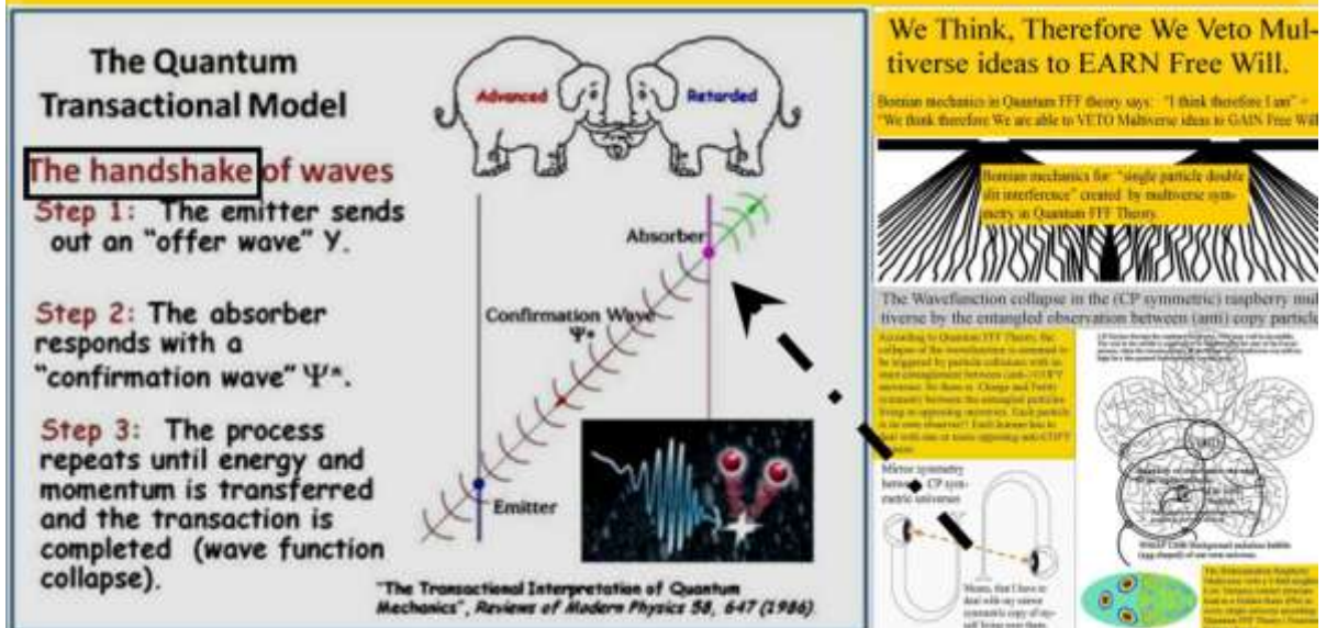
Figure 3, TI handshake in the SuSy Raspberry Multiverse of Q-FFF Theory.
