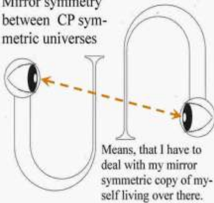
Figure 5, wavefunction collapse between CP symmetric mirror particles by instant entanglement between multi universal bubbles located around the Big Bang central void.
