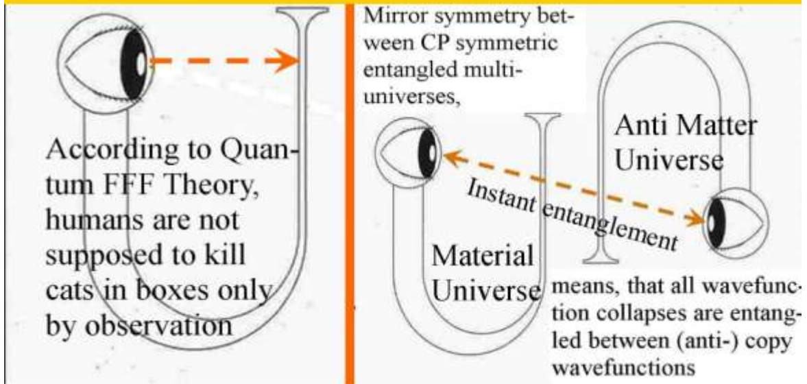
Figure 9. Entanglement between many symmetric universes, needed for the guidance memory of all particles.
