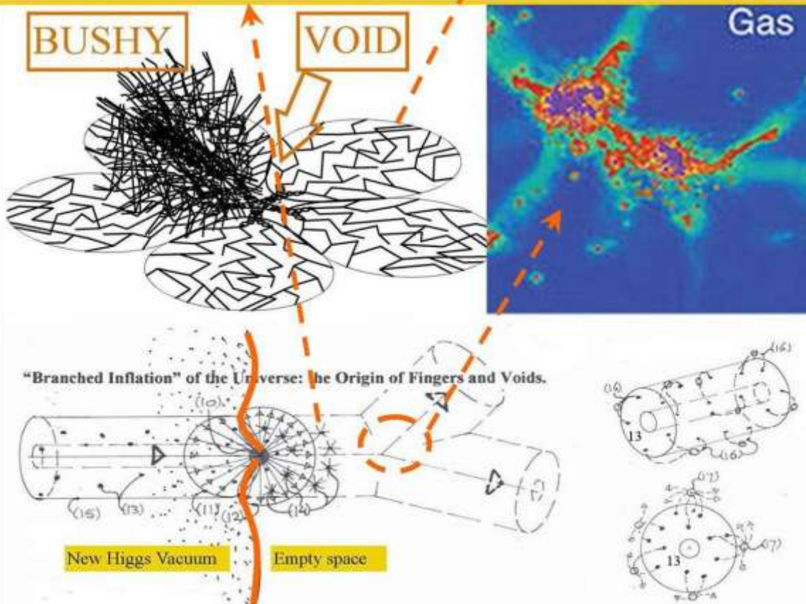
Figure 7, The SuSY explosion of the Big Bang Black Hole splintering into entangled smaller BHs and evaporating into 8 or 12 SuSY oscillating Axion Higgs Vacuum lattices and Dark Matter Black Hole Fractals .
