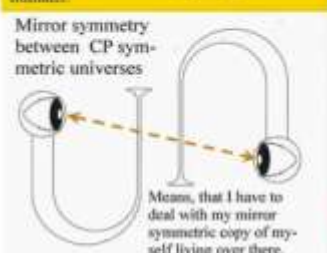
Figure 8, Schrödinger's cat paradox solved with Anti Matter Copy Cats, living inside Entangled Raspberry Multiverse Bubbles
