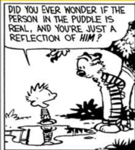
Figure 8, Schrödinger's cat paradox solved with Anti Matter Copy Cats, living inside Entangled Raspberry Multiverse Bubbles
