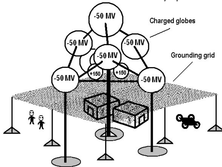
Figure 12.1 Schematic of a popular NASA radiation shield design. Figure redrawn from [1].
