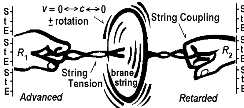
Figure 12.12 Conceptualization of the spin tension-coupling dynamics of a 2-brane spacetime element representing one of the 6^5 paths of Fig. 12.11.
