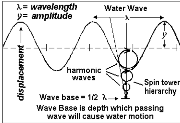
Figure 12.5 Dynamics of water-waves. Water remains stationary as waves pass through. Ocean surface waves are a combination of transverse and longitudinal waves; thus surface points follow orbital paths as in the HAM spacetime model.
