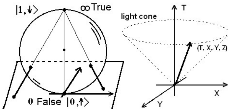
Figure 12.8 a) Block sphere rendition of a qubit. b) Relativistic qubit or r-qubit with more degrees of freedom.
