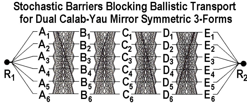
Figure 12.11 A Quantum Calabi-Yau spacetime brane array with 6^5 possible locked paths acting as a barrier to ballistic transport by stochastically disrupting the mean-free-path. The array must be programmed as a harmonic oscillator resonance hierarchy to order the topology coherently.
