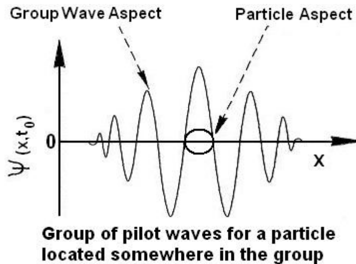
Figure 12.18 The group velocity of de Broglie waves is associated with the velocity of a particle.
