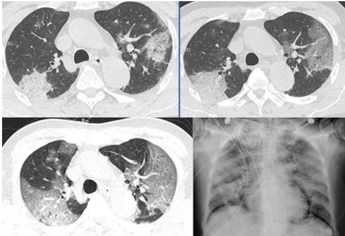
CT traces disease progression in novel coronavirus
