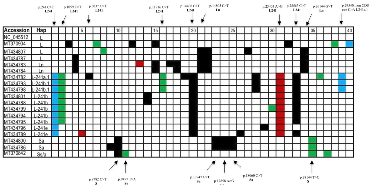
Figure 8 Variable site plot of SNV in each aligned sequence in an 18 sequence alignment for collections New York Mar 5 – 9 versus the Hu-1 ref NC_045512.2. Variable site number across the top, and Sequence ID down left hand side and Haplotype. The
