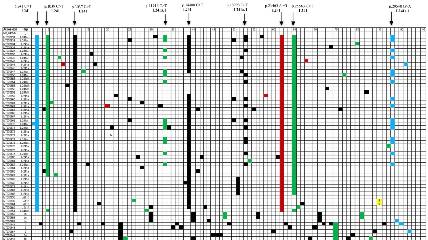
Figure 10 Variable site plot of SNV in each aligned sequence in a 58 sequence alignment for collections New York Mar 14 – 19 versus the Hu-1 ref NC_045512.2. Variable site number across the top, and Sequence ID down left hand side and Haplotype. The
